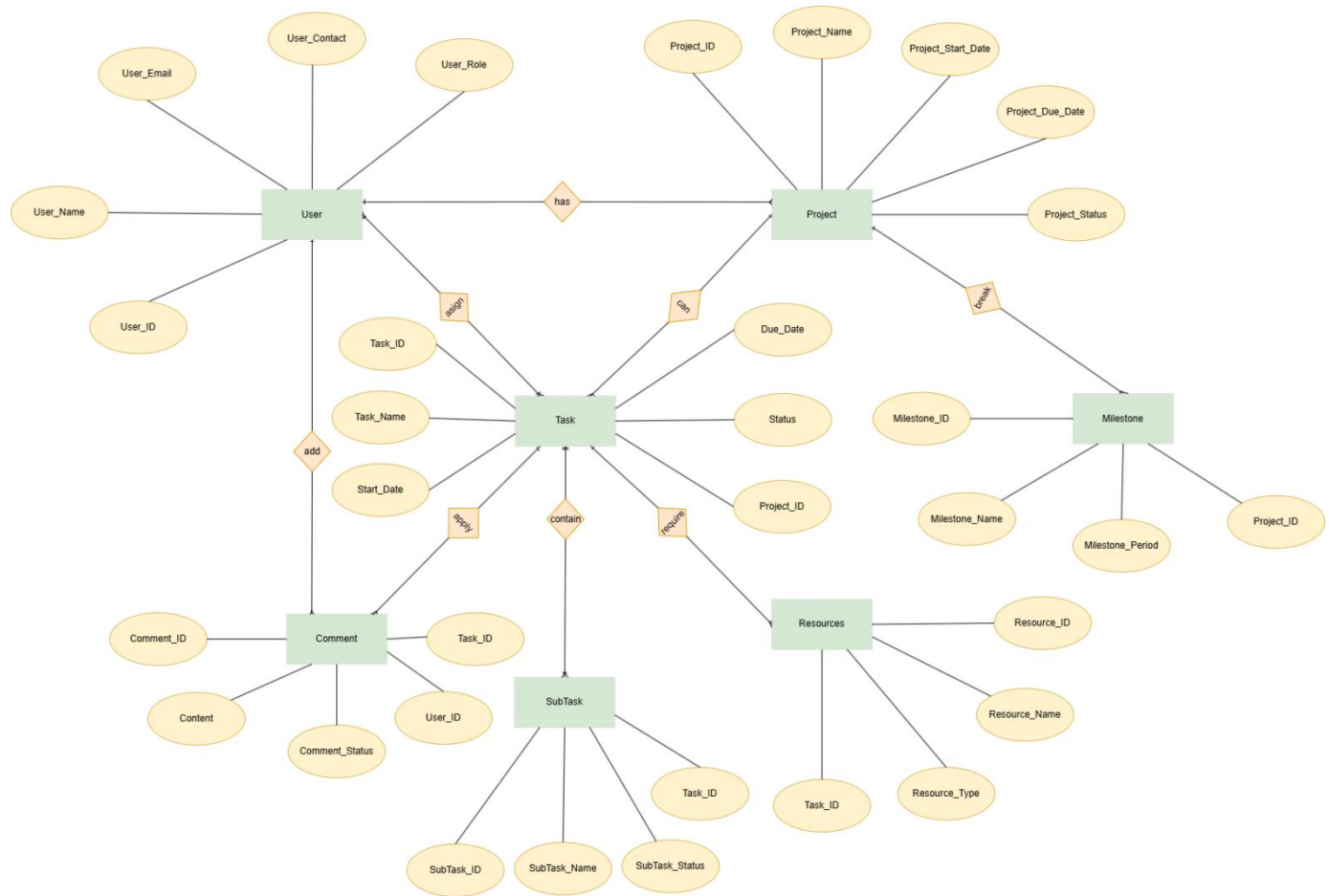
Figure 1 Initial ERD
