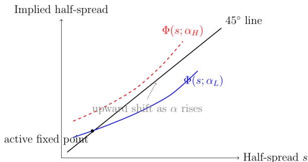
Figure 2: Schematic fixed-point representation. As AI penetration rises from \alpha_L to \alpha_H , the implied-spread operator shifts upward. The figure is illustrative only and does not impose
