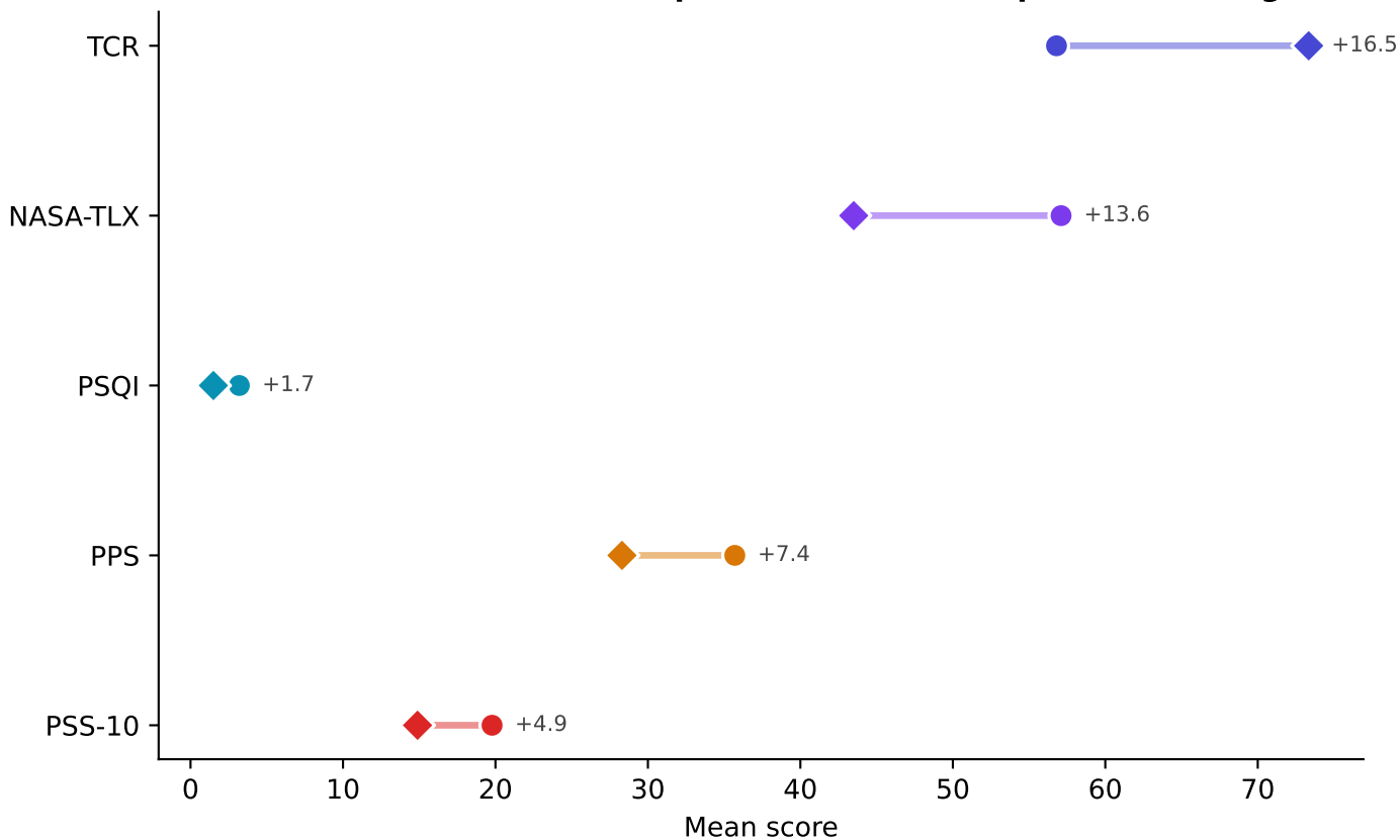
Figure 4.3 — Mean Change by Metric (N = 10)
