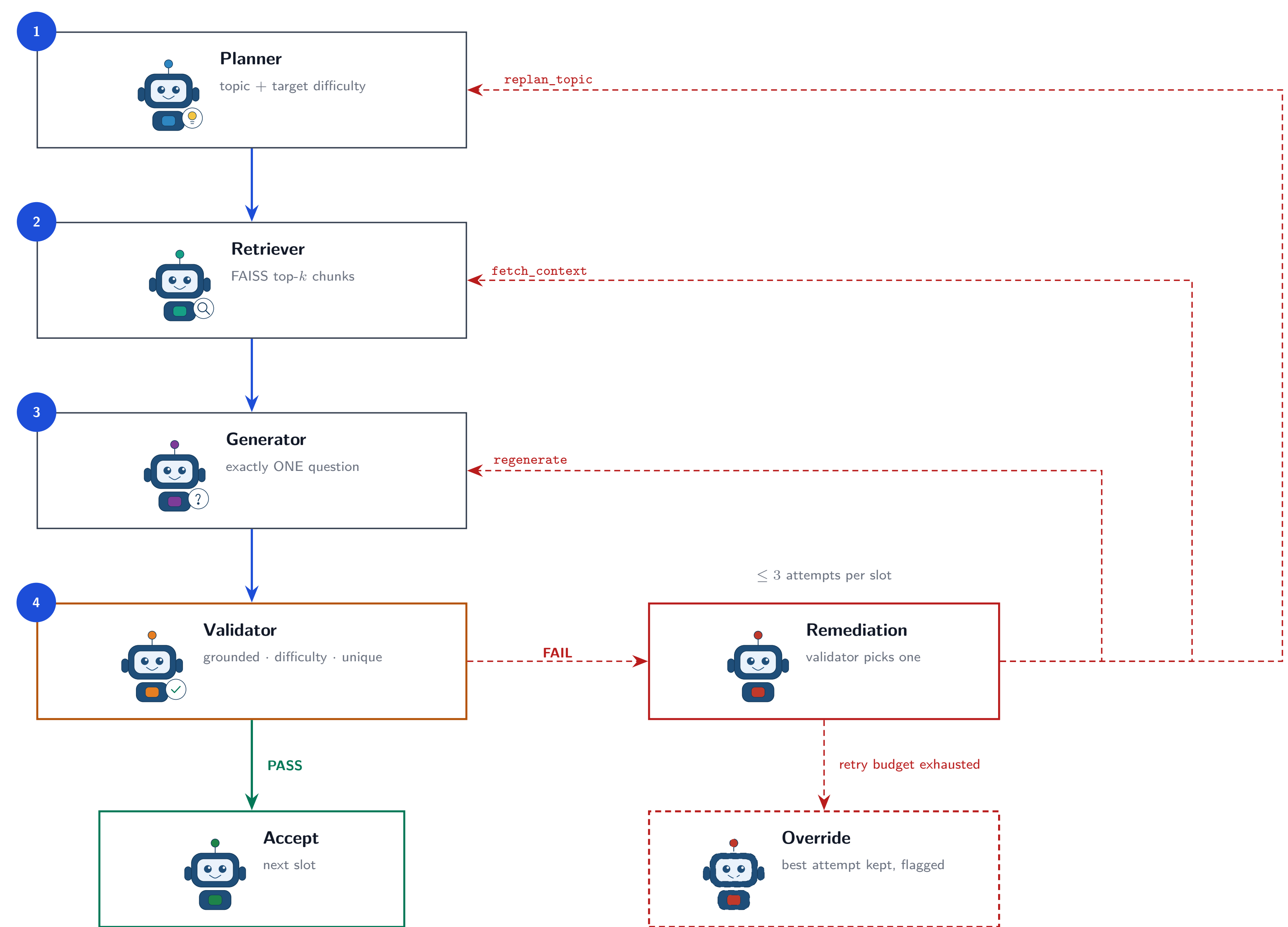
Figure 4. One question per slot; each must pass validation before the next begins. An exhausted retry budget flags an override, never a pass.
