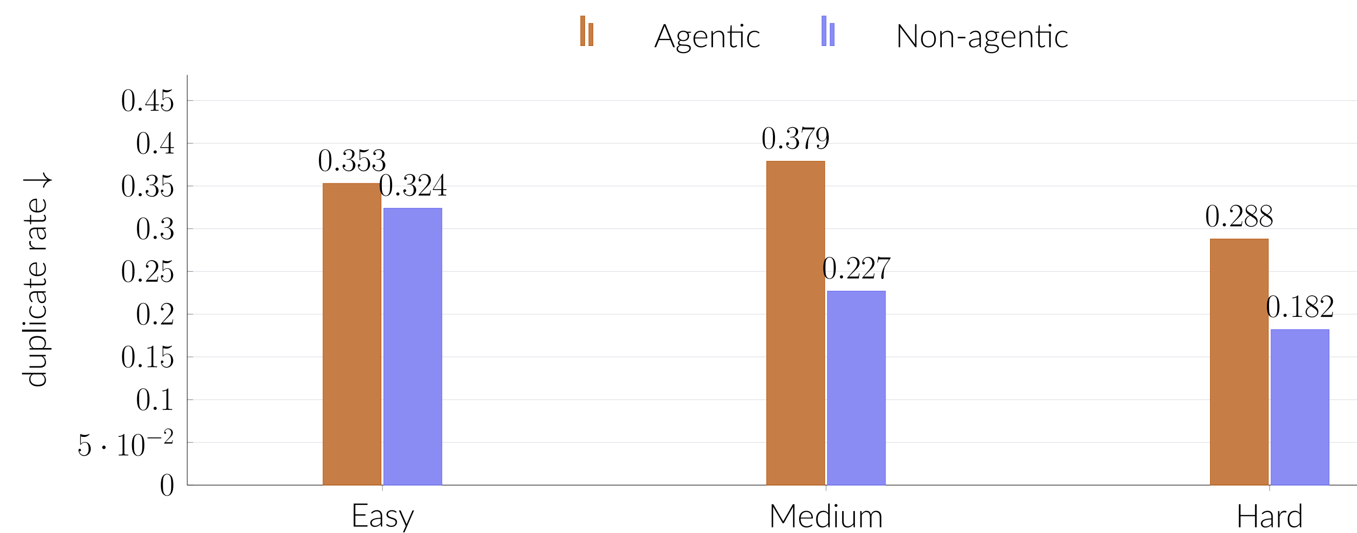
Figure 6. Duplicate rate by difficulty — the agentic loop duplicates more in every band.
