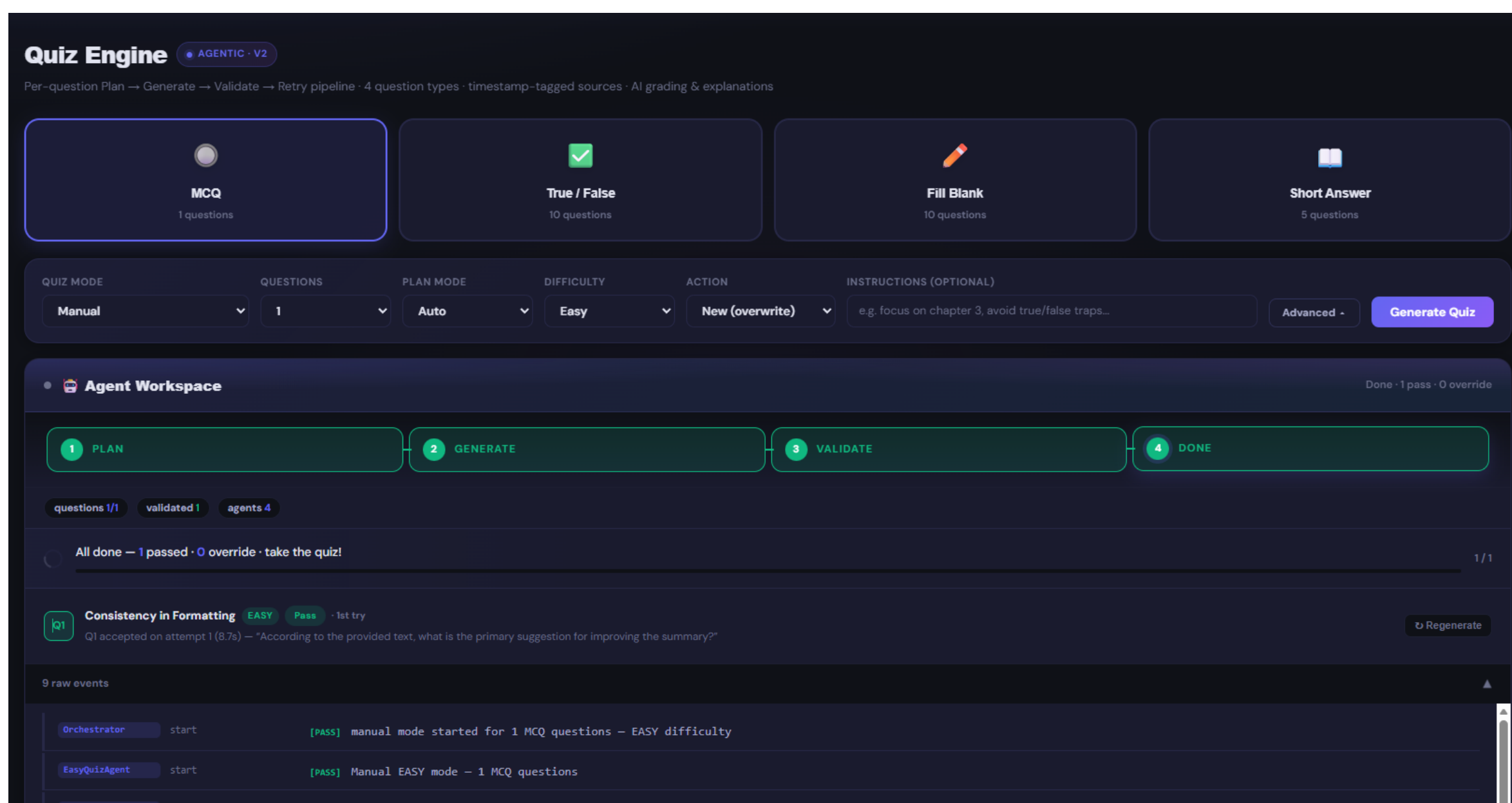
Figure 2. After a run. The Agent Workspace shows the loop of Figure 4 completing — Plan, Generate, Validate, Done — with live counters ( questions 1/1, validated 1, agents 4 ), the per-question verdict and attempt time, and the raw agent event log beneath.
