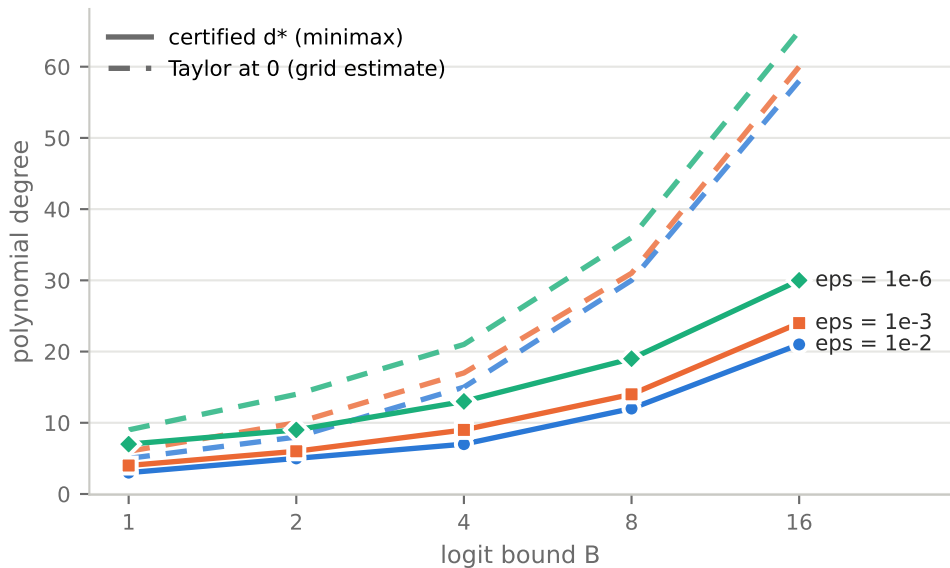
Certified minimal degree (solid) vs Taylor degree (dashed)
