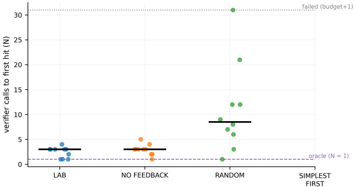
Replay y_{\text{inf}} (lattice), 10 seeds; bar = median
