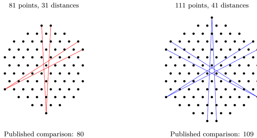
Figure 1: Exact lattice constructions on the same drawing scale. Colored segments show all four pairs at squared distance 91 (left) and all six pairs at 127 (right). Comparison counts refer to Ahmed–Snevily (2013).
