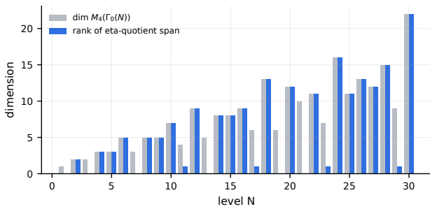
Fig. 4 Exact comparison, for every level N \leq 30 , of \dim M_4(\Gamma_0(N)) (grey) with the rank of the span of all holomorphic eta-quotients of weight 4 with trivial character (blue).
