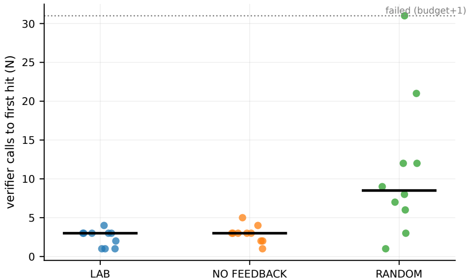
Replay y_{\text{inf}} (lattice), 10 seeds; bar = median
