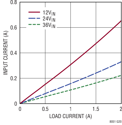
Input vs Load Current V_{OUT} = 5\text{V} , 2MHz, BIAS = 5V, Burst Mode
