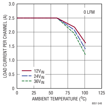
Single Channel Derating, V OUT = 5V CH1 ON, CH2/CH3/CH4 OFF BIAS = 5V, DC2860A Demo Board T J = 120°C, Burst Mode
