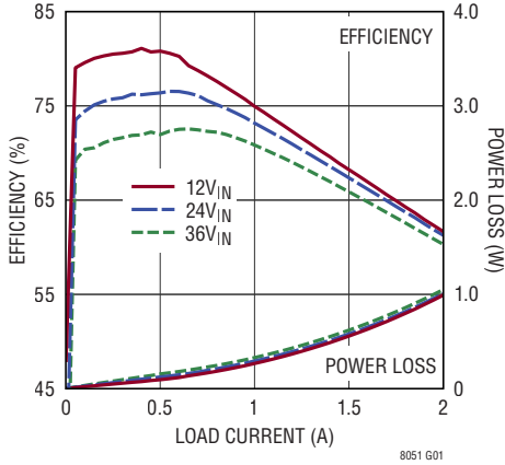
Efficiency, V_{OUT} = 0.8\text{V} BIAS = 5V
