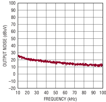
Output Noise Spectrum DC2860A, 100kHz Span V_{IN} = 12\text{V} , V_{OUT} = 3.3\text{V} I_{OUT} = 1.2\text{A} , f_{SW} = 1.2\text{MHz}
