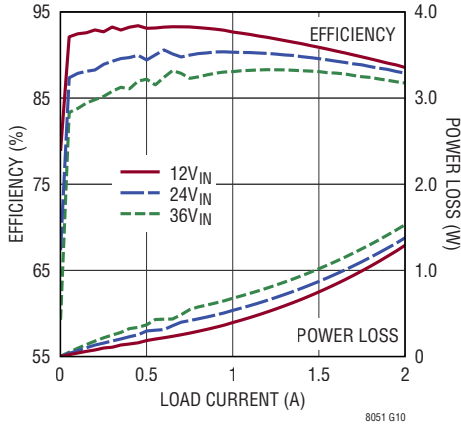
Efficiency, V_{OUT} = 5.0\text{V} BIAS = 5V, Burst Mode
