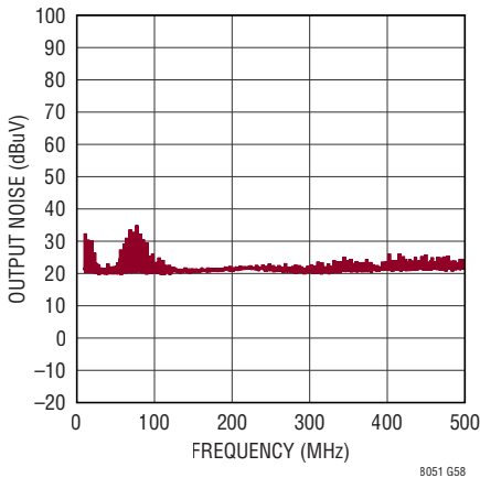
Output Noise Spectrum DC2860A, 500MHz Span V_{IN} = 12\text{V} , V_{OUT} = 3.3\text{V} I_{OUT} = 1.2\text{A} , f_{SW} = 1.2\text{MHz}
