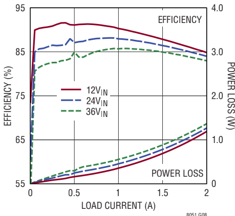
Efficiency, V_{OUT} = 3.3\text{V} BIAS = 5V, Burst Mode
