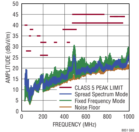
CISPR25 Radiated Emission with Class 5 Peak Limit DC2860A Demo Board, V_{IN} = 14\text{V} , V_{OUT} = 3.3\text{V} Four Channels Paralleled, I_{OUT} = 4.8\text{A} , f_{SW} = 2\text{MHz}
