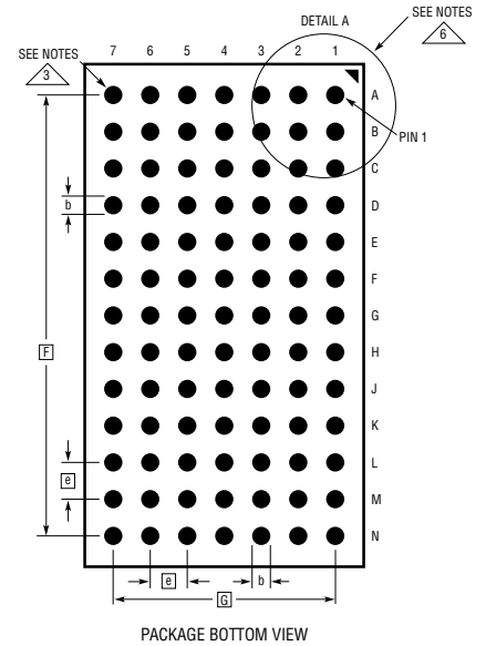
PACKAGE BOTTOM VIEW
