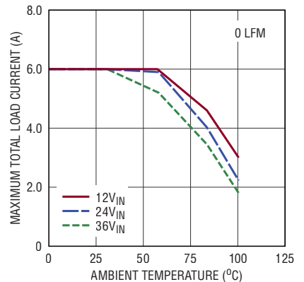
Derating, V_{OUT} = 3.3\text{V} , F_{SW} = 2\text{MHz} BIAS = 5V, DC2860A Demo Board T_J = 120^\circ\text{C} , Burst Mode All Channels At Same Load
