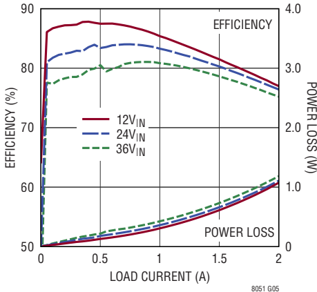
Efficiency, V_{OUT} = 1.8\text{V} BIAS = 5V, Burst Mode
