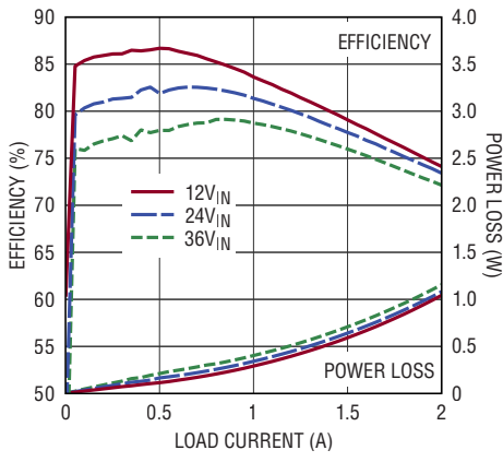
Efficiency, V_{OUT} = 1.5\text{V} BIAS = 5V, Burst Mode
