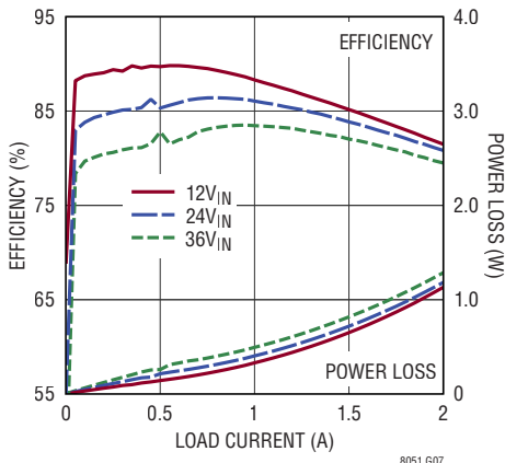
Efficiency, V_{OUT} = 2.5\text{V} BIAS = 5V, Burst Mode
