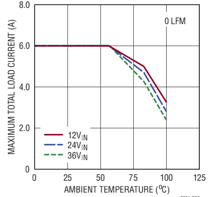
Derating, V_{OUT} = 2\text{V} BIAS = 5V, DC2860A Demo Board T_J = 120^\circ\text{C} , Burst Mode All Channels At Same Load
