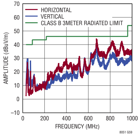
CISPR22 Class B Emissions DC2860A Demo Board V_{INn} = 12\text{V} , I_{OUTn} = 1.2\text{A} 5V_{OUT1} , 3.3V_{OUT2} , 2.5V_{OUT3} , 1.8V_{OUT4} Spread Spectrum On, No EMI Filter
