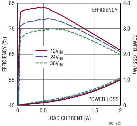
Efficiency, V_{OUT} = 1.0\text{V} BIAS = 5V, Burst Mode
