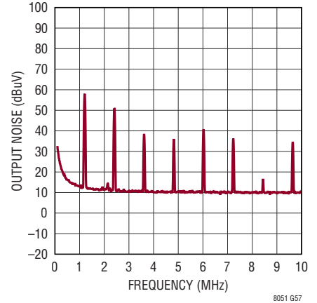
Output Noise Spectrum DC2860A, 100MHz Span V_{IN} = 12\text{V} , V_{OUT} = 3.3\text{V} I_{OUT} = 1.2\text{A} , f_{SW} = 1.2\text{MHz}
