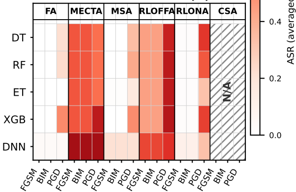
(b) Missed-attack ASR_{[FN]}
