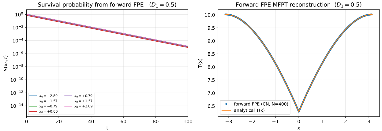
Figure 4: Left : survival probability S(x_0, t) obtained from the Crank–Nicolson forward FPE solver, for seven different starting positions and D_1 = 0.5 ; the log-linear plot confirms exponential decay at long times. Right : the MFPT T(x_0) recovered from \int_0^\infty S dt (plus an exponential-tail correction) matches the analytical formula (17).
