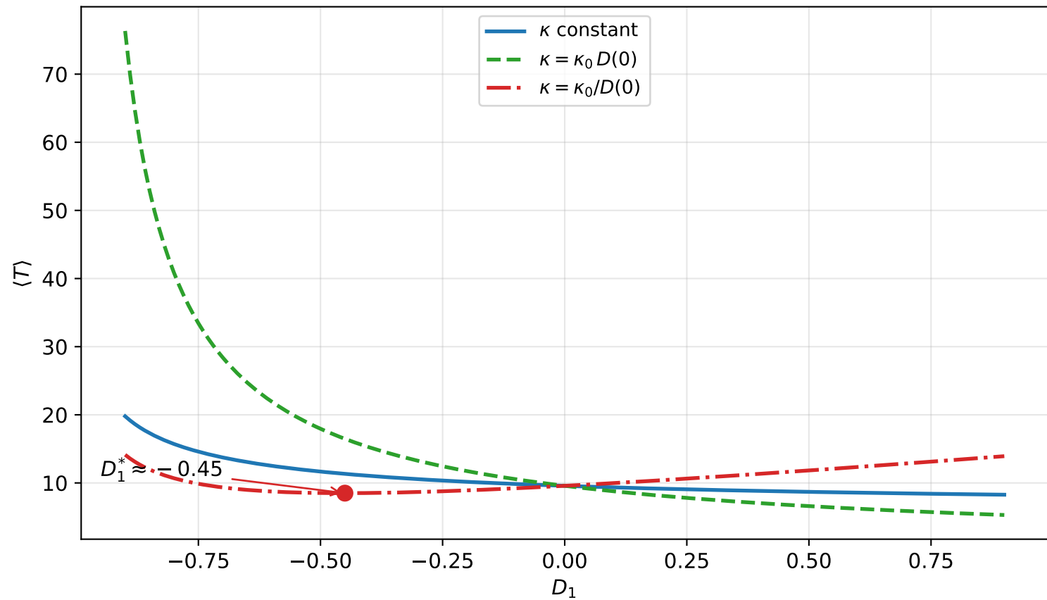
Three microscopic stories for \kappa(D(0)) ( D_0 = 1, \kappa_0 = 1 )
