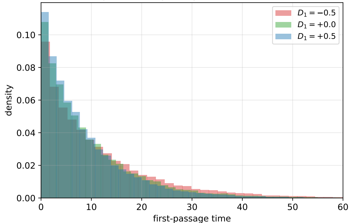
Empirical first-passage time distributions
