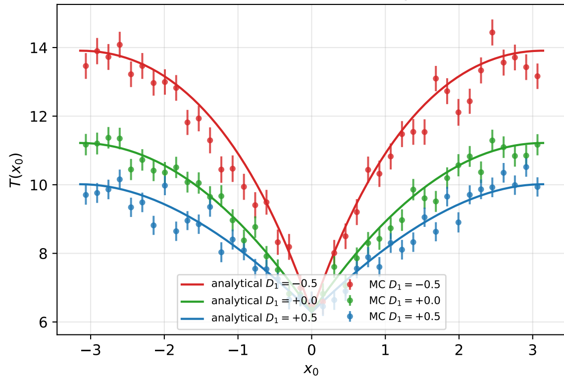
Monte Carlo MFPT vs. analytical
