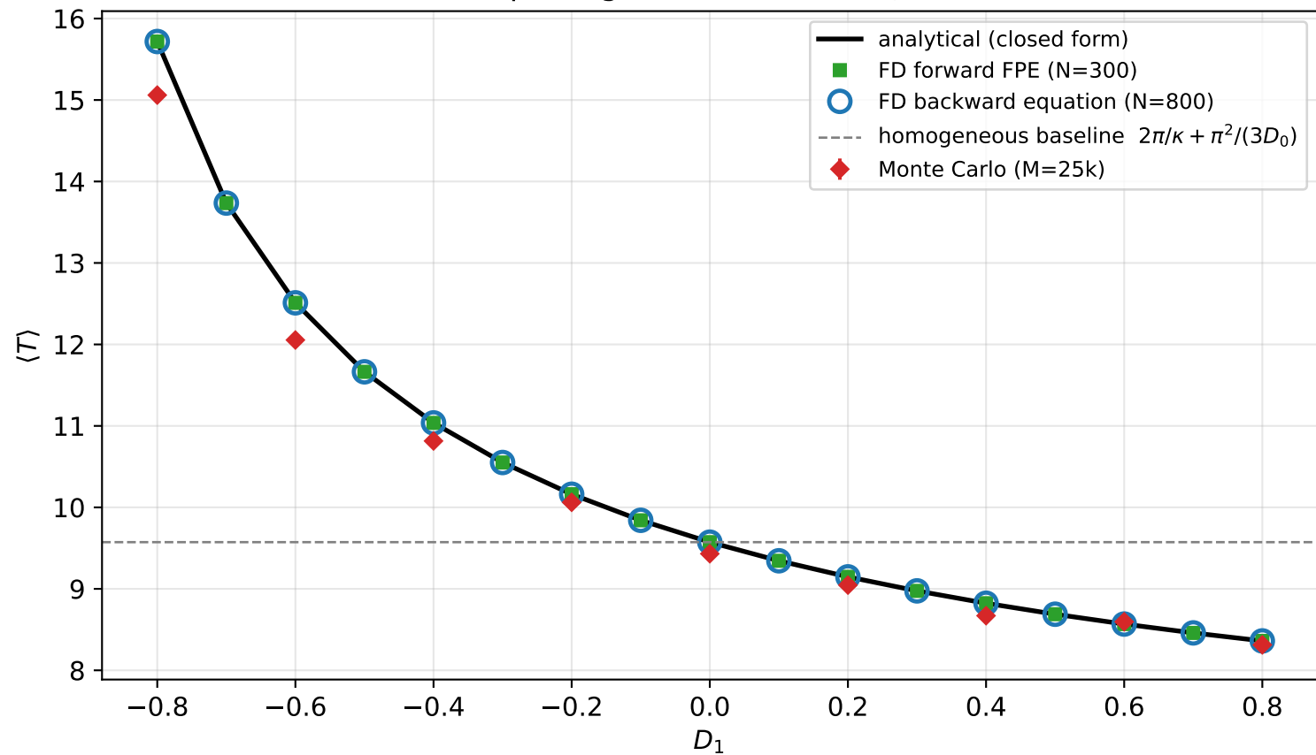
Mean first-passage time vs. D_1 ( D_0 = 1 , \kappa = 1 )
