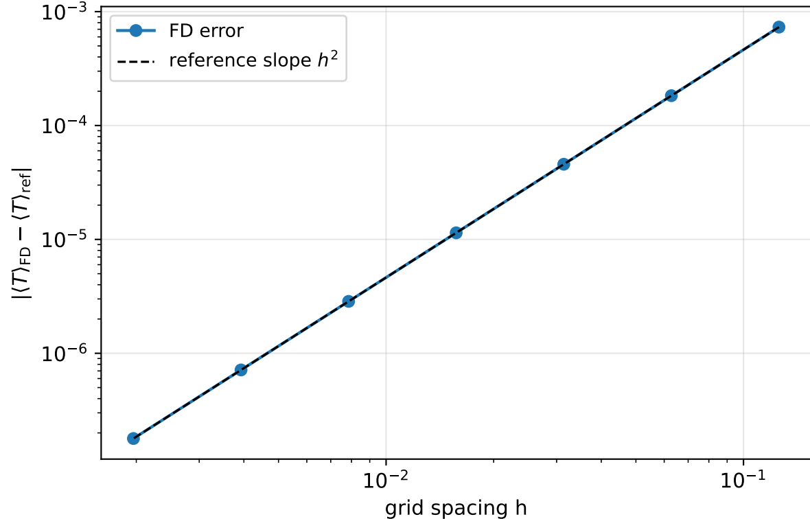
FD backward-equation convergence ( D_1 = 0.5 )
