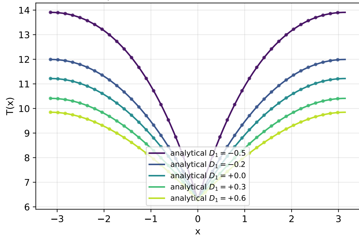
Backward-equation MFPT: closed form vs. finite difference
