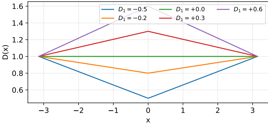
Tent diffusivity profile D(x) = D_0 + D_1(1 - |x|/\pi)
