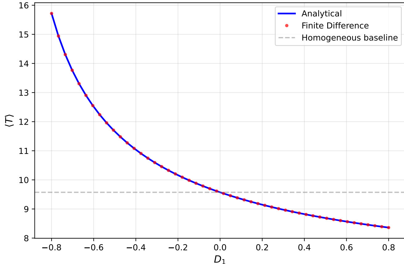
Average MFPT vs D_1
