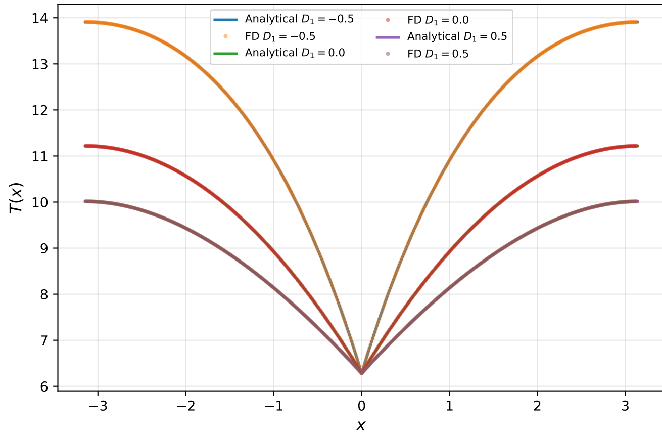
MFPT T(x) : Analytical vs Finite Difference
