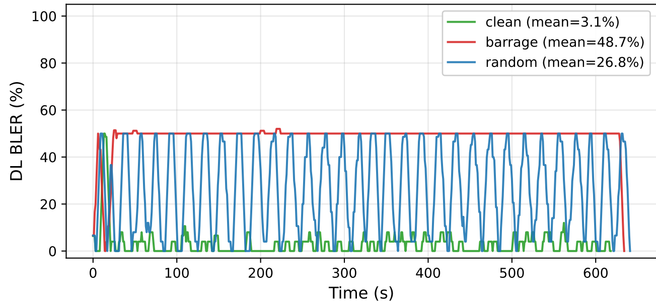
Downlink Block Error Rate per class
