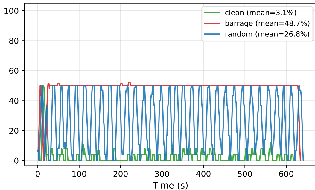
(a) Downlink BLER signature per class
