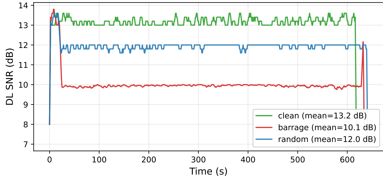
Downlink SNR per class
