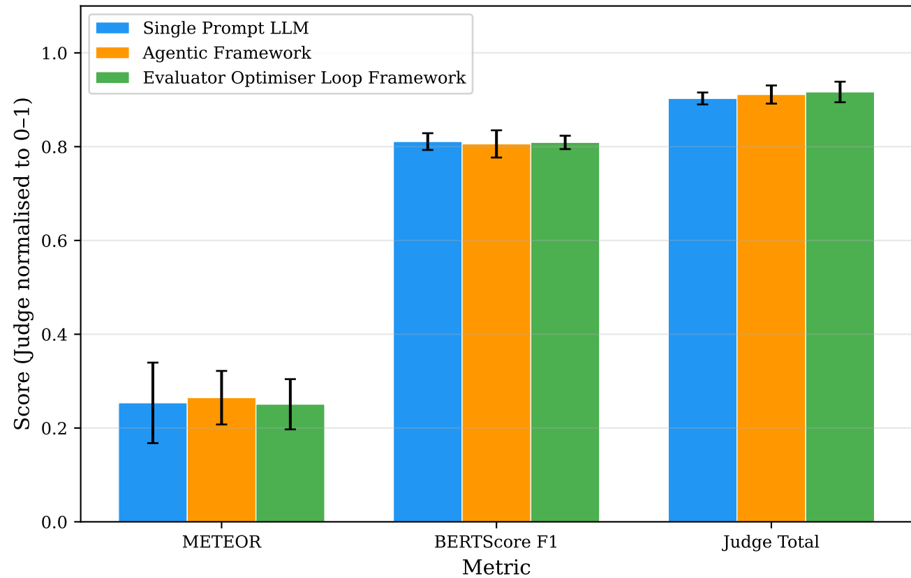
Version Comparison — Average Across All Models
