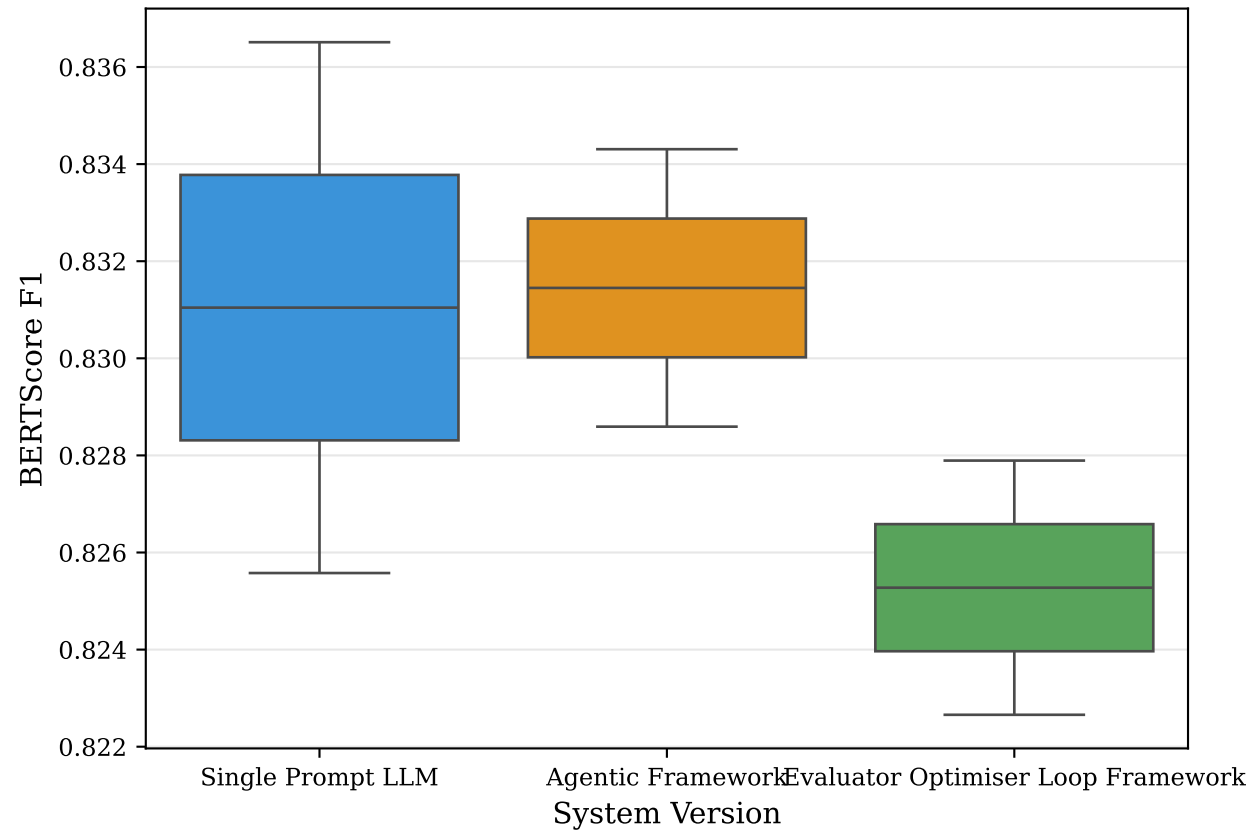
BERTScore F1 Distribution by Version (Gemini 3.1 Pro)
