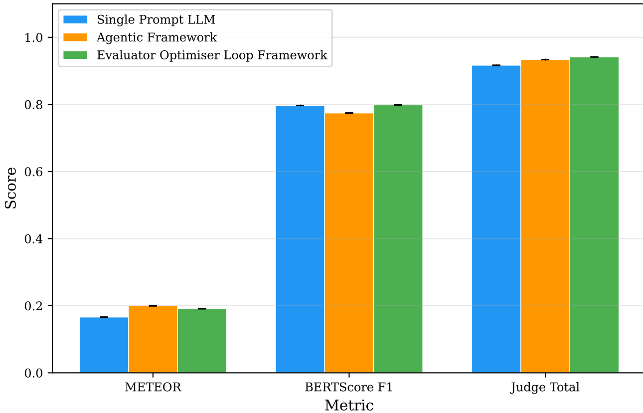
Version Comparison (Claude Sonnet 4.6)
