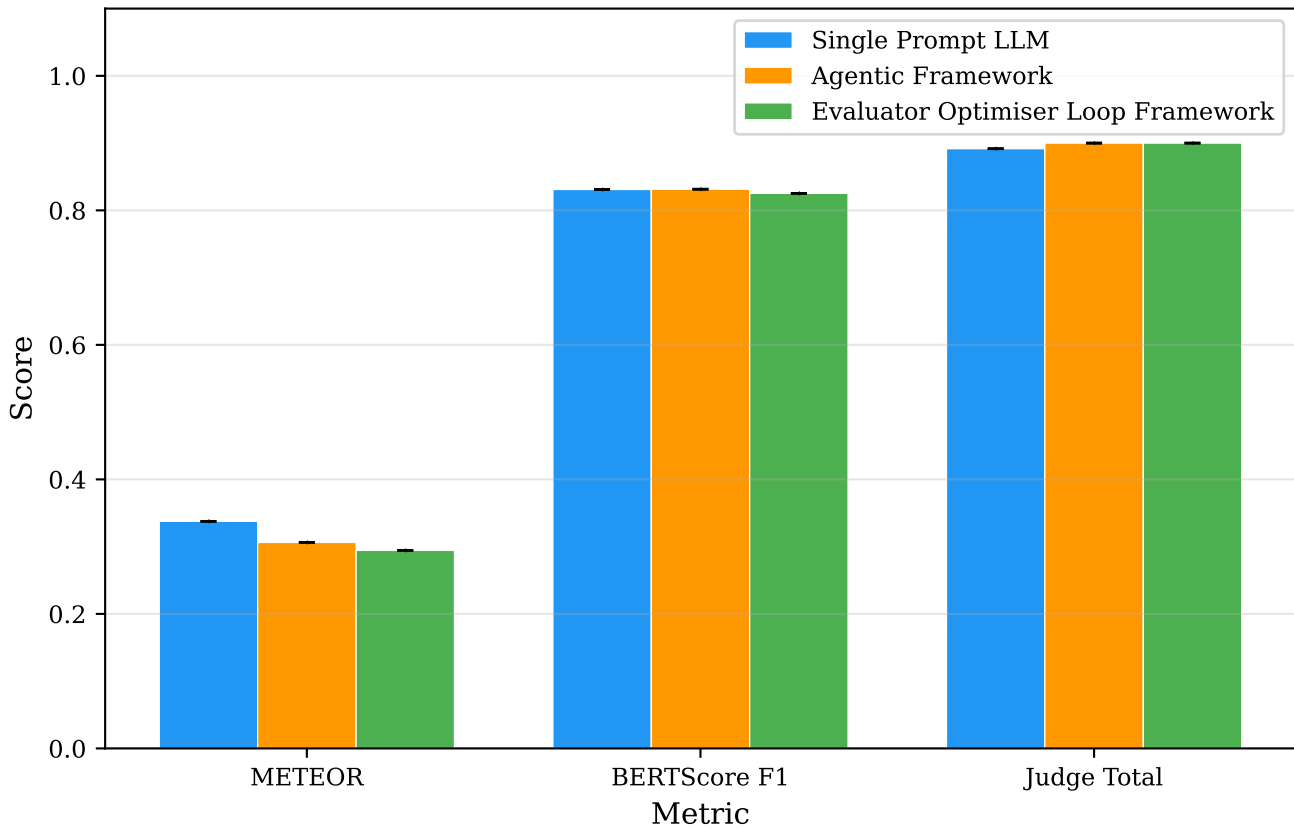
Version Comparison (Gemini 3.1 Pro)
