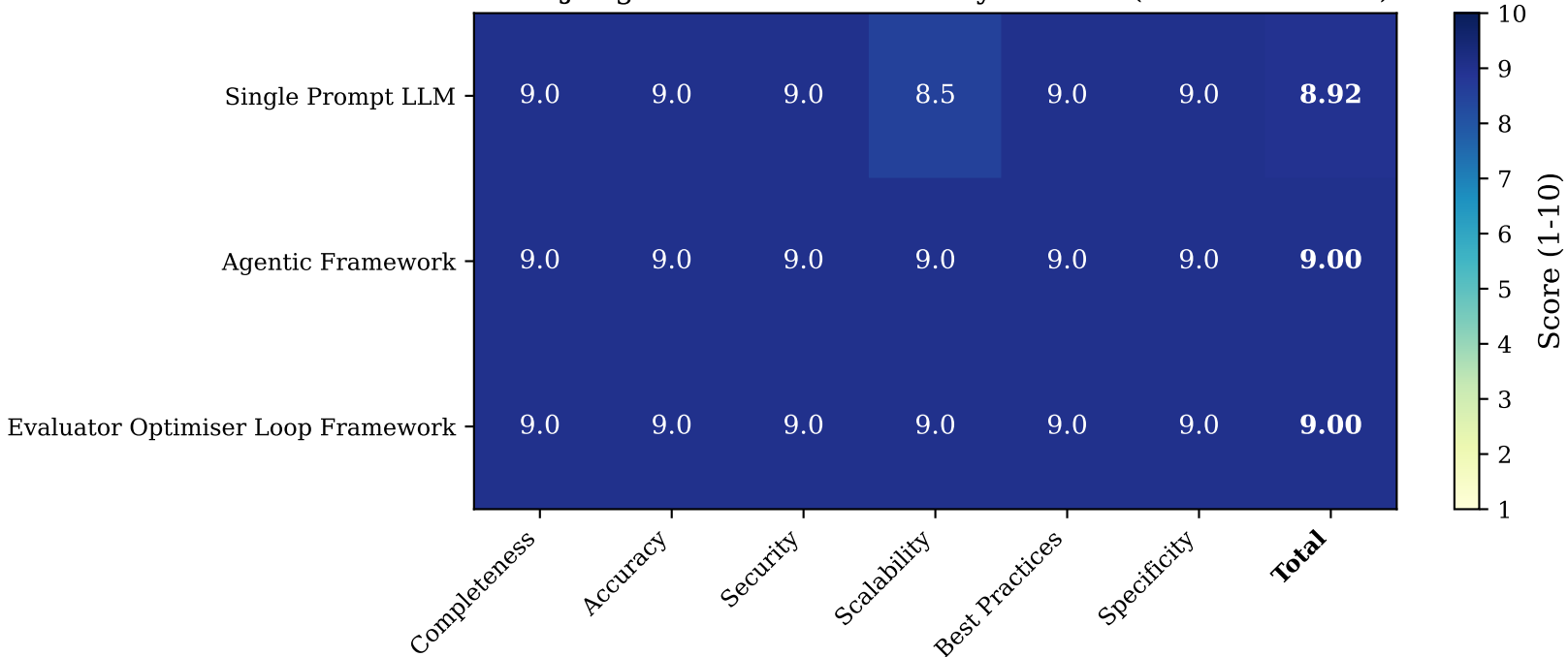
LLM Judge Dimension Scores by Version (Gemini 3.1 Pro)
