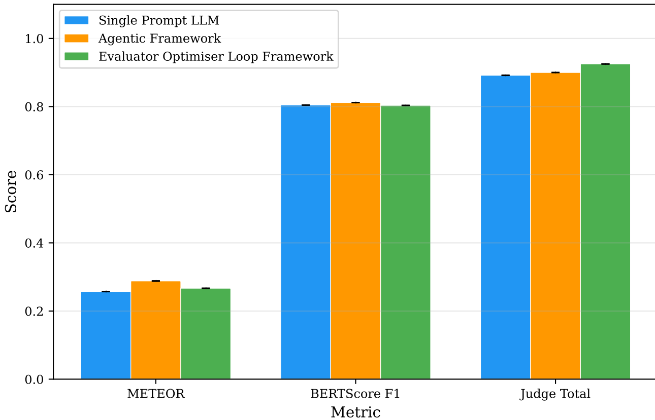
Version Comparison (GPT-5.4)
