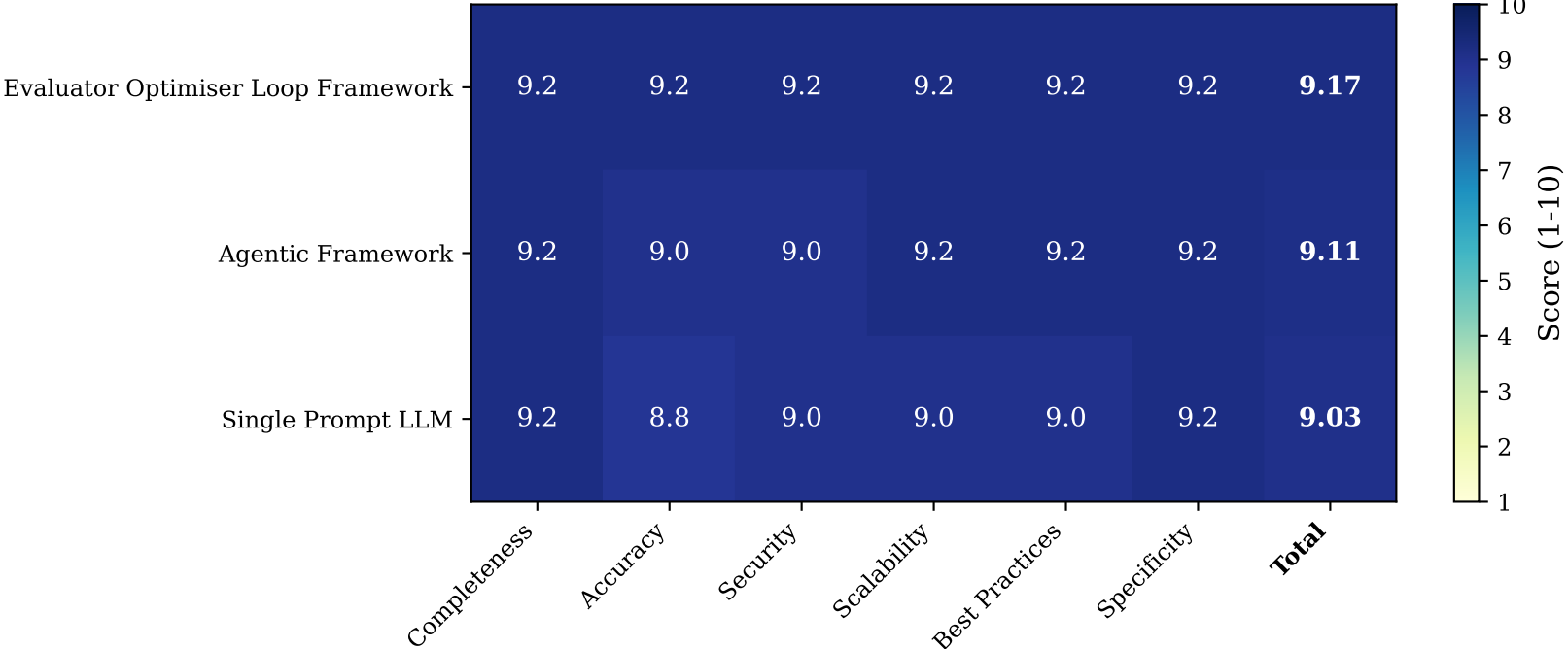
LLM Judge Dimension Scores by Version (All LLMs Combined)
