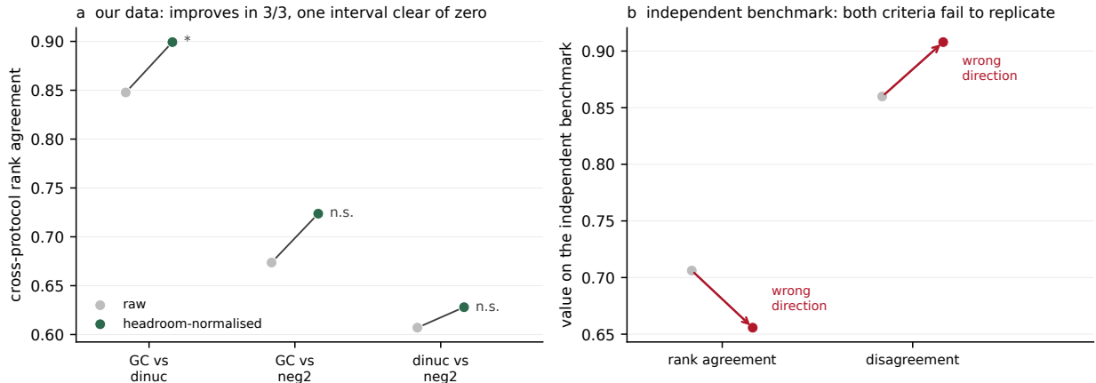
Figure 6: The recommendation, and where it stops working. (a) On our data, cross-protocol rank agreement before and after dividing by the baseline’s headroom, for each protocol pair. Agreement improves in 3 of 3, but only the GC-versus-dinucleotide improvement has a protein-clustered interval clear of zero. (b) The same test on the independent benchmark of Figure 5, n = 45 : rank agreement falls and disagreement rises under normalisation, which are the two criteria pre-registered as falsifying the recommendation. The change in rank agreement is -0.050 [ -0.222, +0.140 ], so this is a failure to replicate rather than a refutation.
