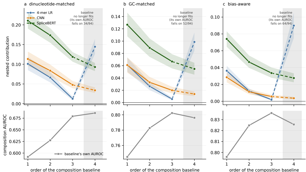
Figure 5: Nested contribution against the order of the composition baseline, n = 94 datasets, in each negative-set protocol: (a) dinucleotide-matched, (b) GC-matched, (c) bias-aware. Top row, contribution for each model class, with 95% protein-clustered percentile intervals as bands; the step from order three to order four is dashed because it crosses out of the range where the baseline is a baseline. Bottom row, the composition baseline’s own out-of-fold AUROC, which is the diagnostic: the shaded region marks order four, where a 337-column block overfits and its own AUROC falls on 34, 52 and 64 of the 94 datasets. The 4-mer’s contribution rises there while the two neural models’ continue to fall, because the order-four block spans the 4-mer’s feature space and its pre-fit score repairs a fit the baseline cannot achieve alone. Panel means can still rise where the per-dataset AUROC falls on a minority of datasets, which is why the counts are given.
