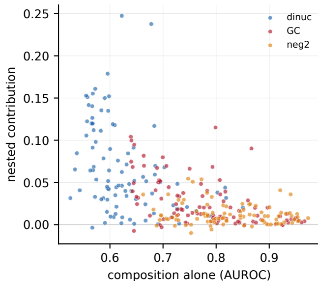
b it tracks the headroom, \rho = -0.60
