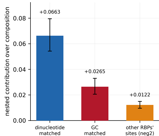
a same model, same positives: 5.4x
