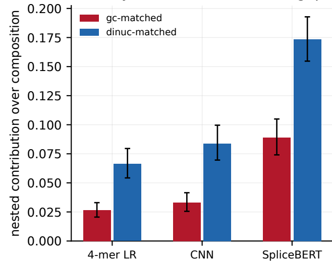
a every model shows the arm gap
