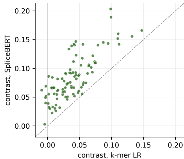
c larger for SpliceBERT in 94/94
