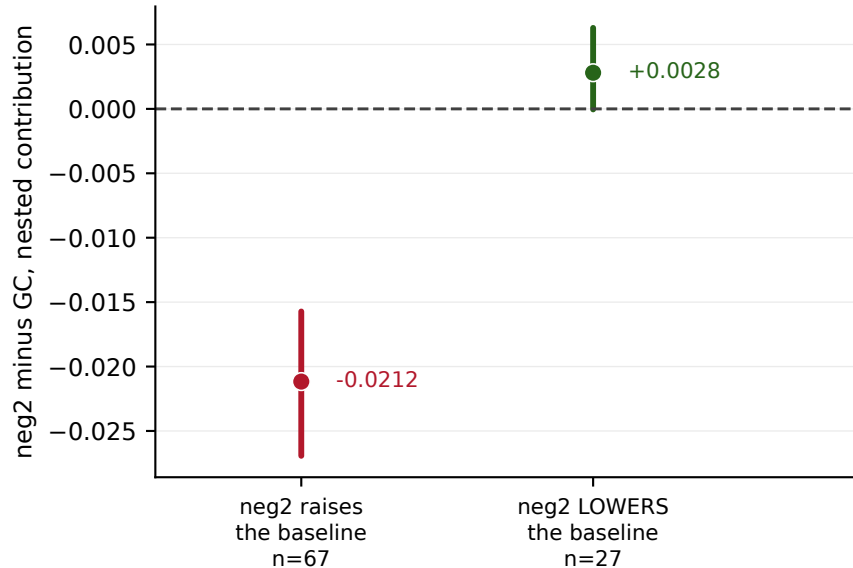
b the deficit follows the baseline, not the label
