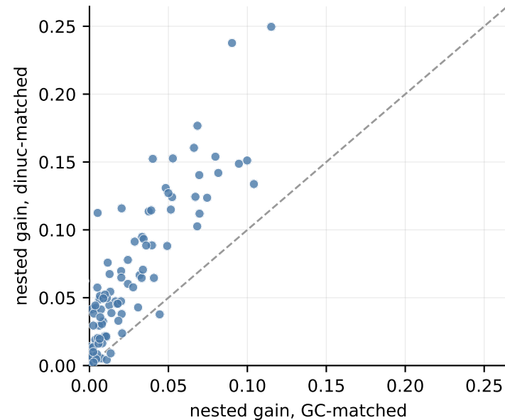
a larger under proper matching in 88/94
