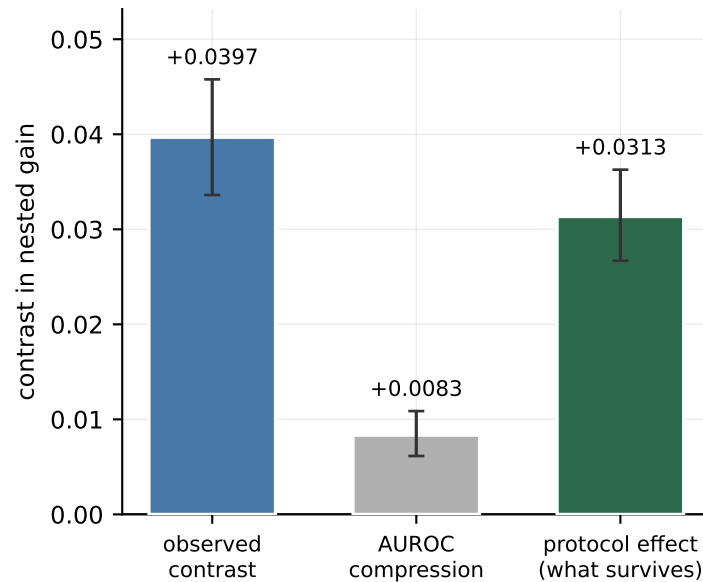
b compression explains 21%, not all of it
