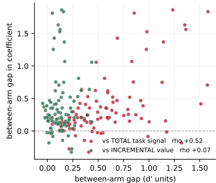
c the coefficient tracks difficulty, not value
