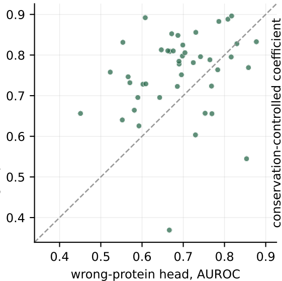
b right wins 33/44, p=3.9e-04
