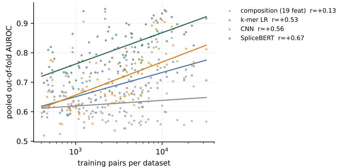
Better models depend MORE on dataset size
