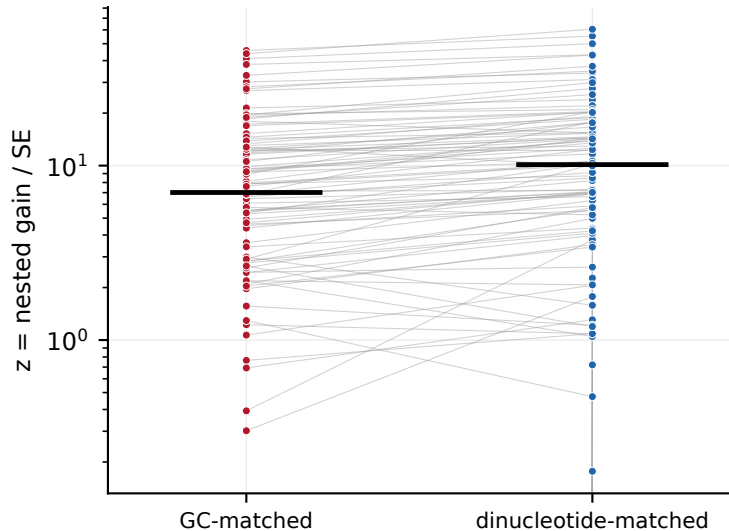
b measured more precisely in 83/94
