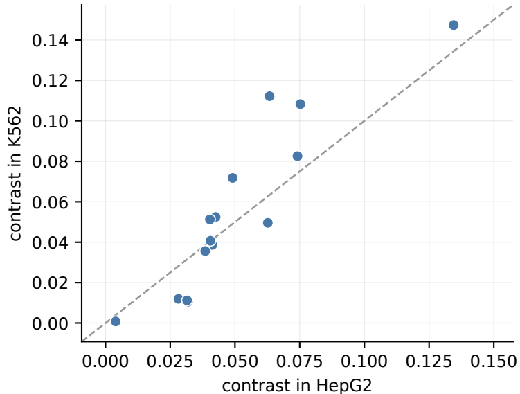
a replicates across cell lines, r = +0.91 (n=15)
