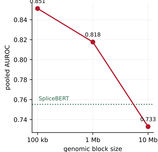
c positional signal decays with block size
