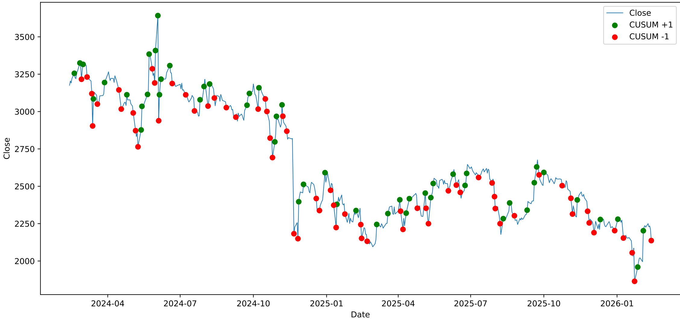
ADANIENT - Close with CUSUM Events
