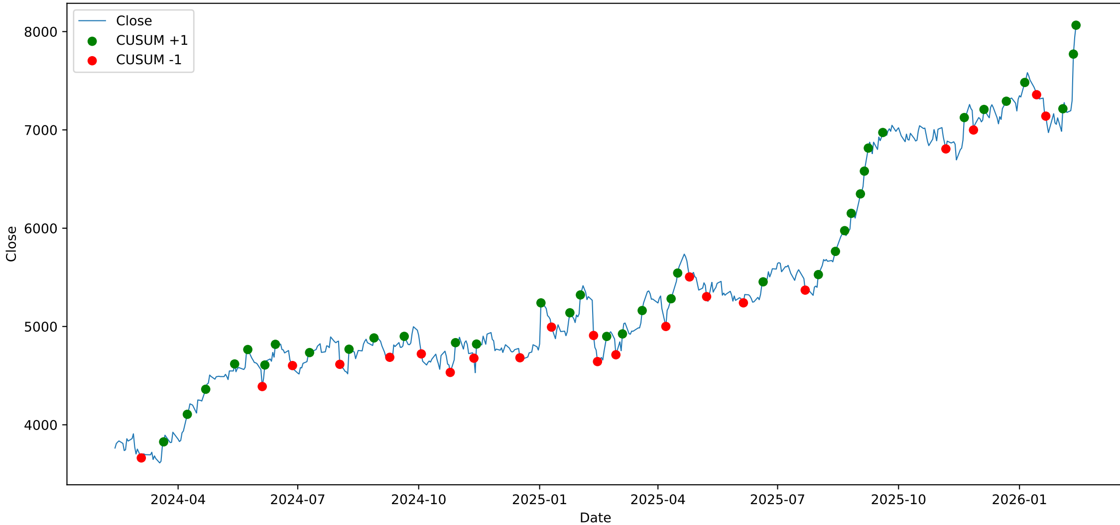
EICHERMOT - Close with CUSUM Events
