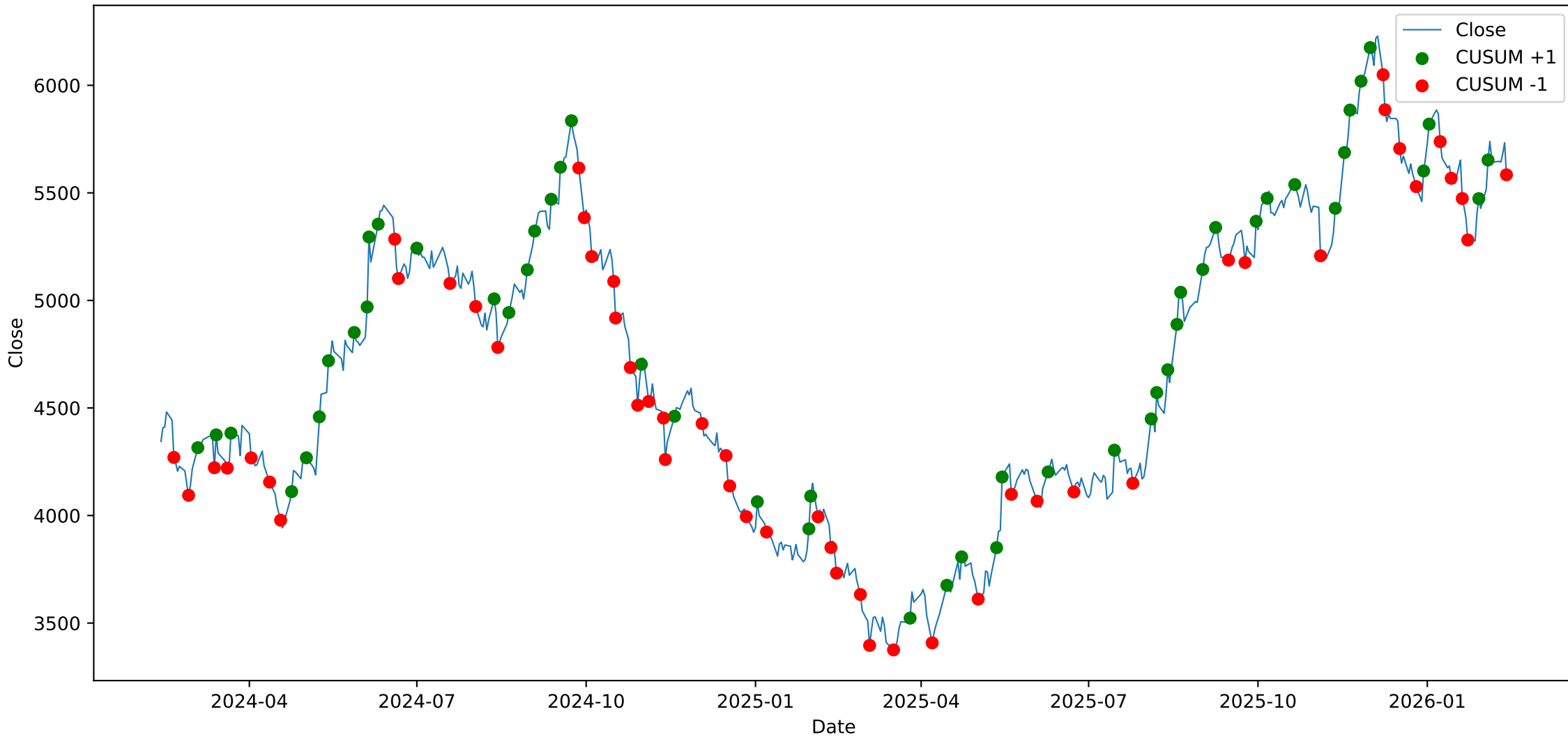
HEROMOTOCO - Close with CUSUM Events
