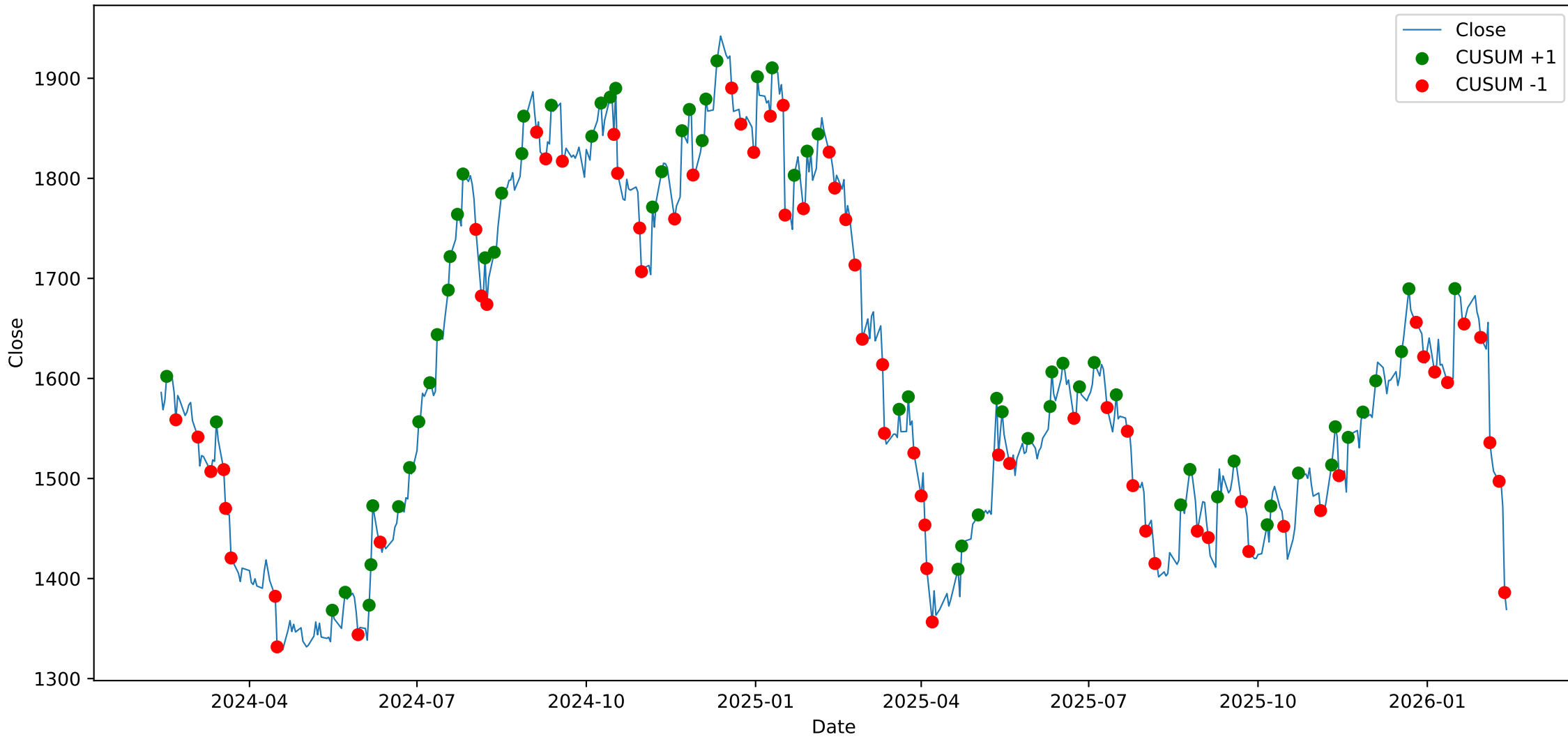
INFY - Close with CUSUM Events
