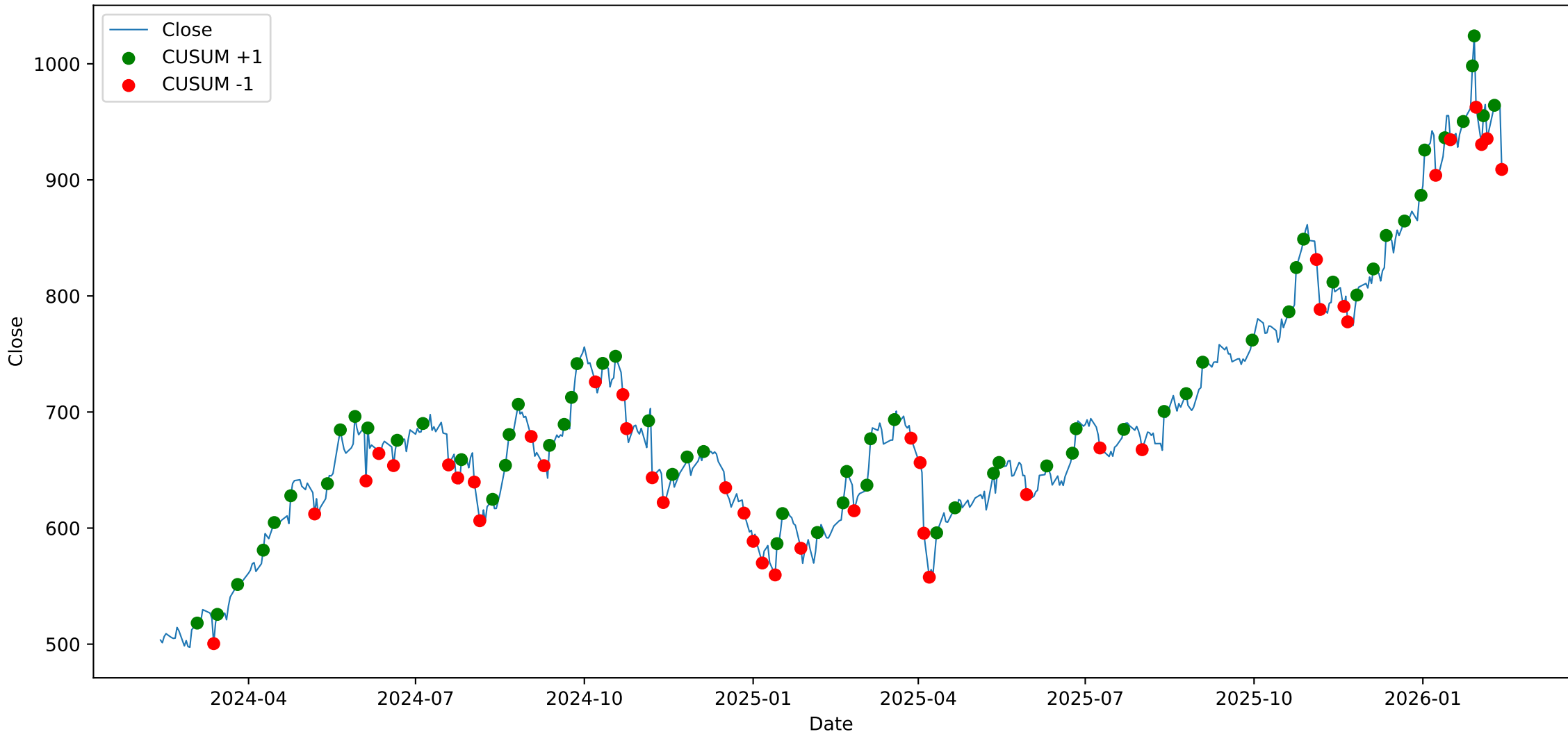
HINDALCO - Close with CUSUM Events
