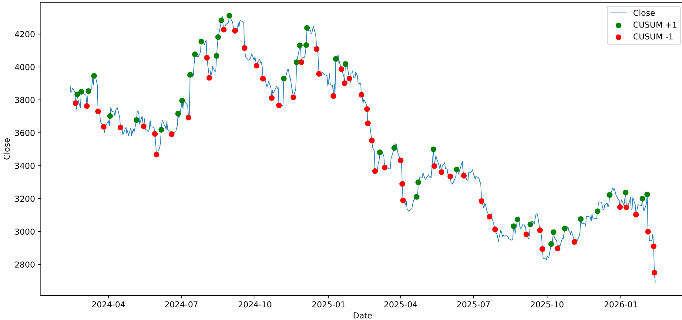
TCS - Close with CUSUM Events
