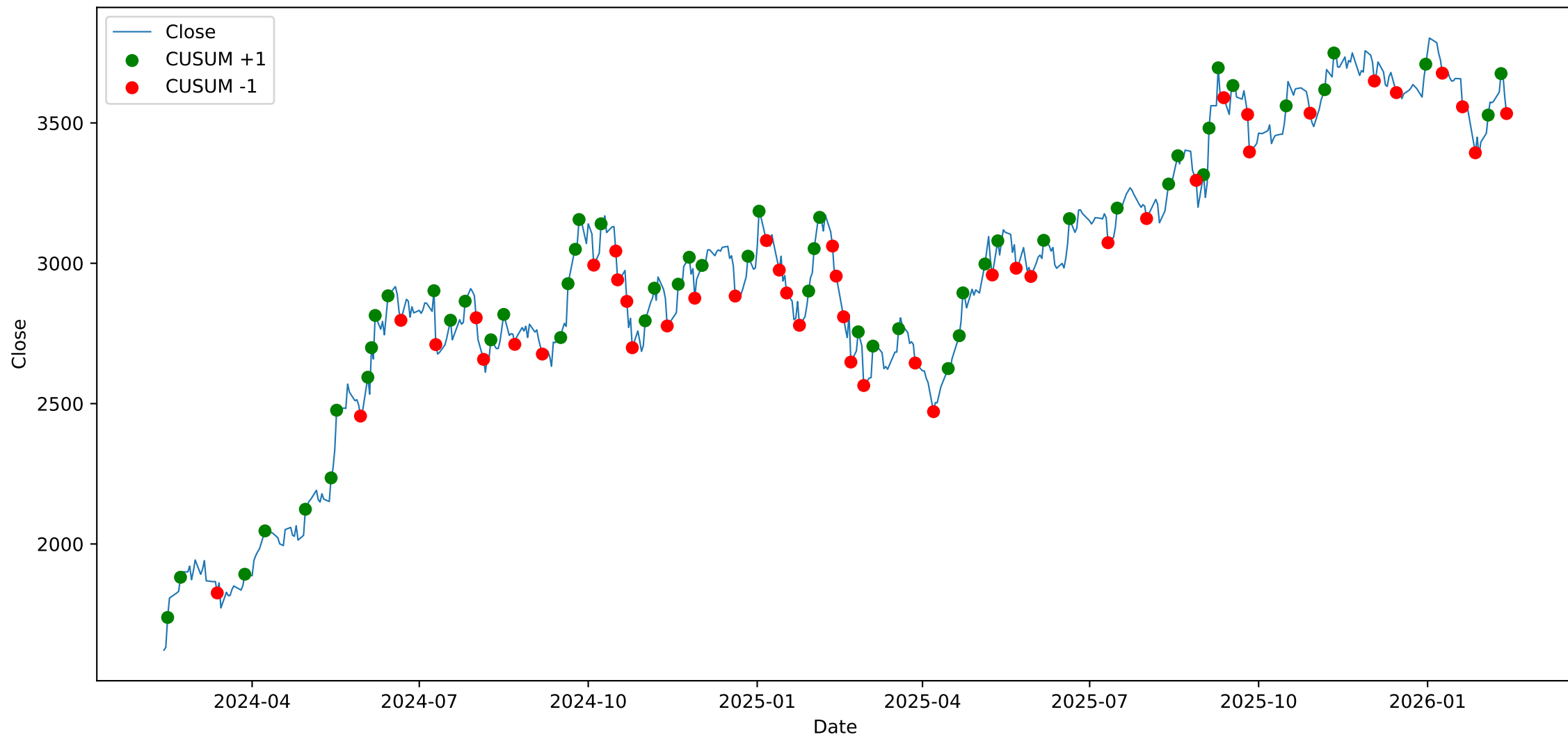
M&amp;M - Close with CUSUM Events
