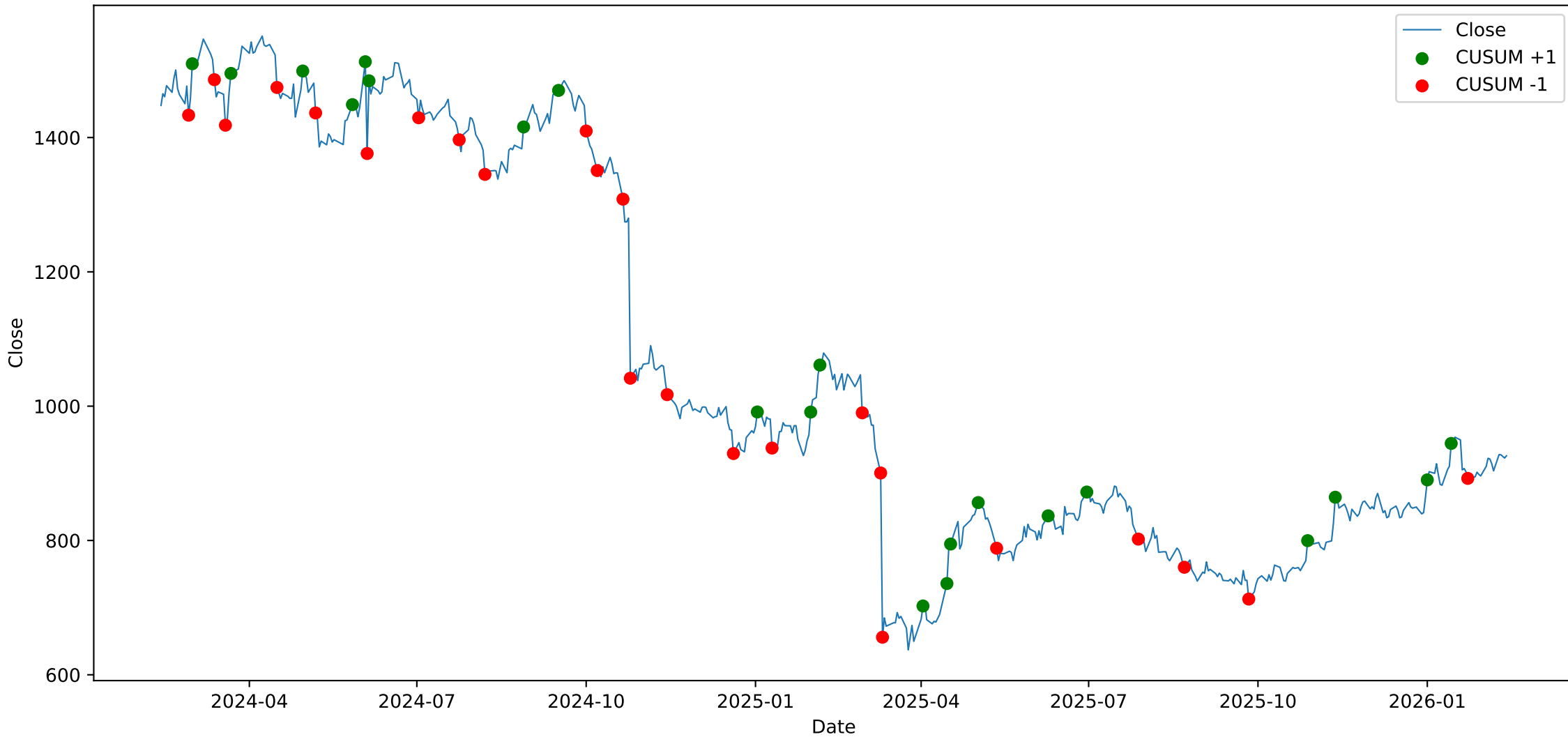
INDUSINDBK - Close with CUSUM Events
