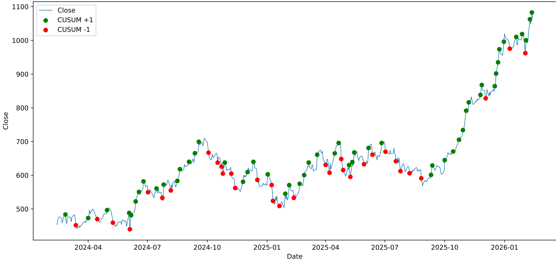
SHRIRAMFIN - Close with CUSUM Events
