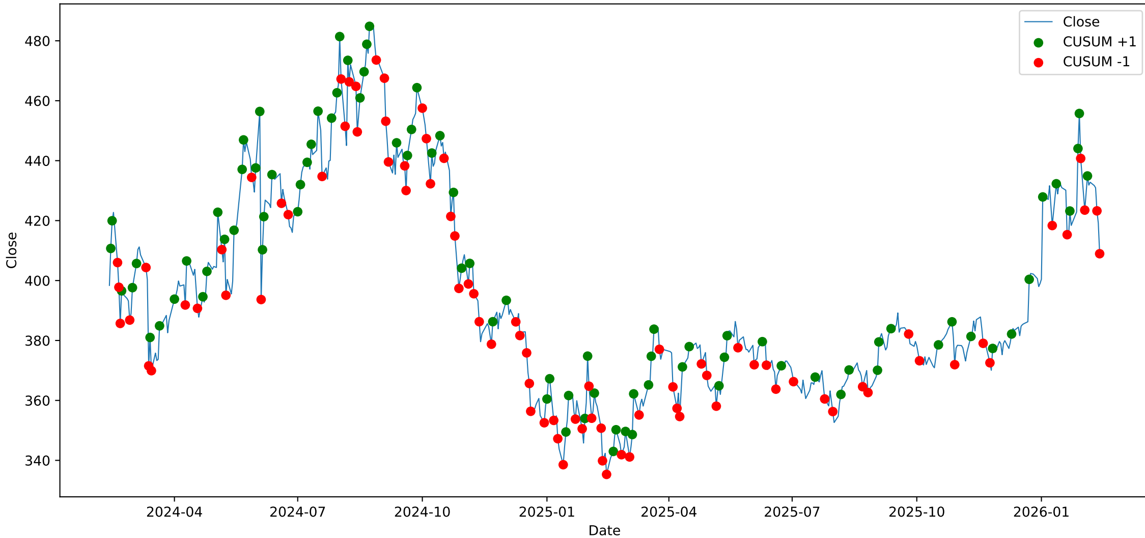
COALINDIA - Close with CUSUM Events
