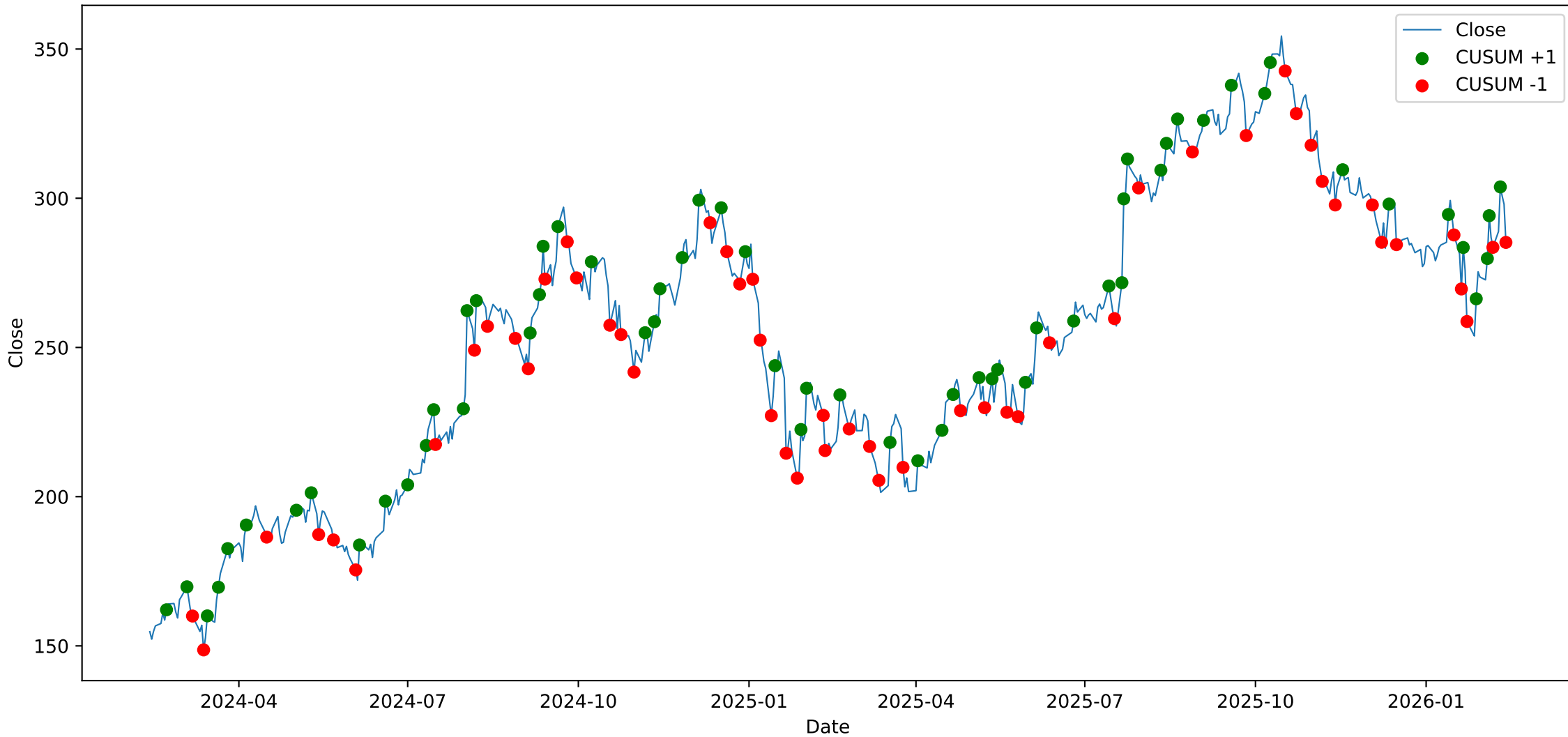
ETERNAL - Close with CUSUM Events
