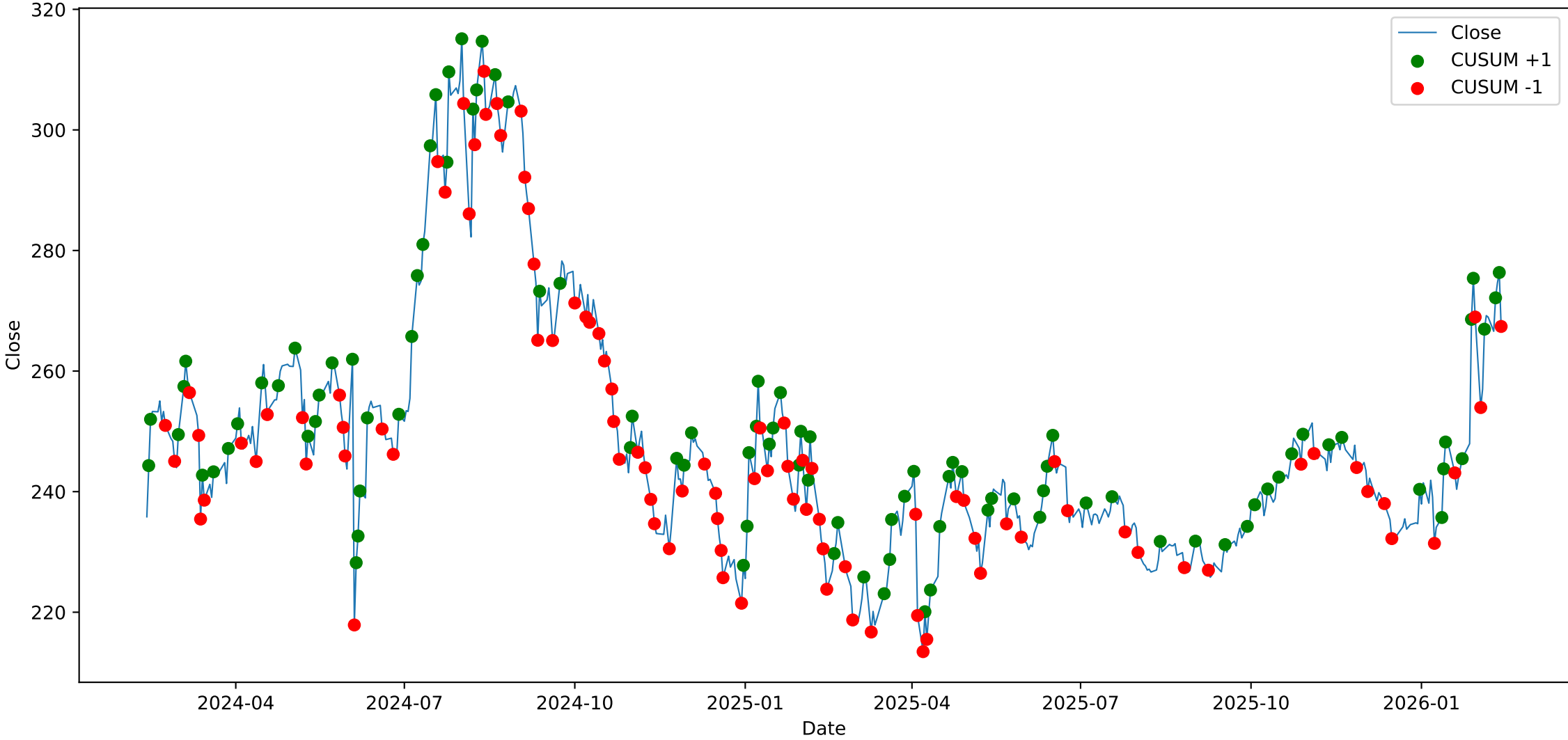
ONGC - Close with CUSUM Events
