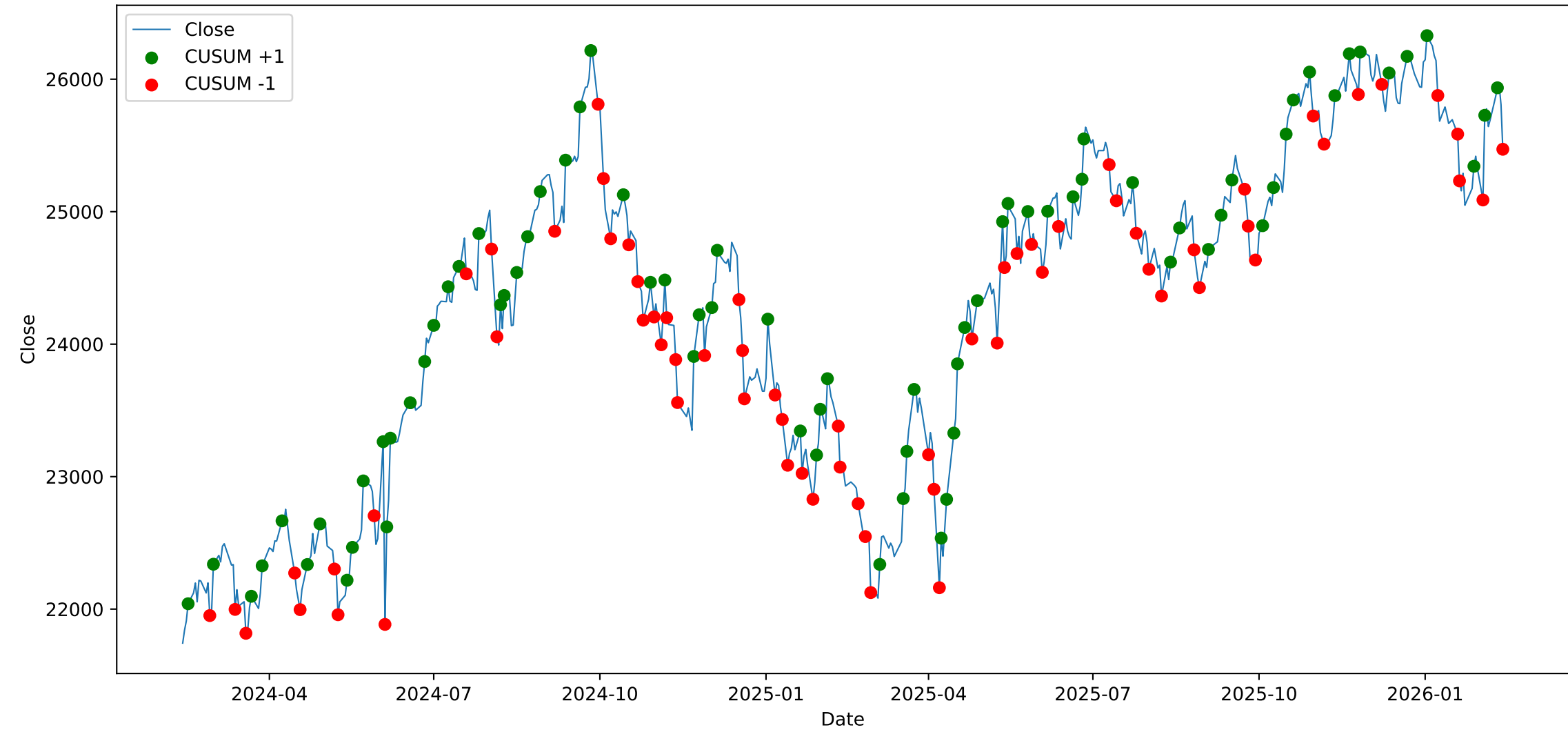
NIFTY - Close with CUSUM Events
