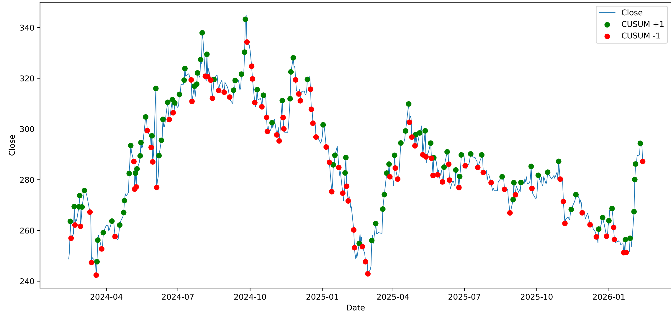
POWERGRID - Close with CUSUM Events
