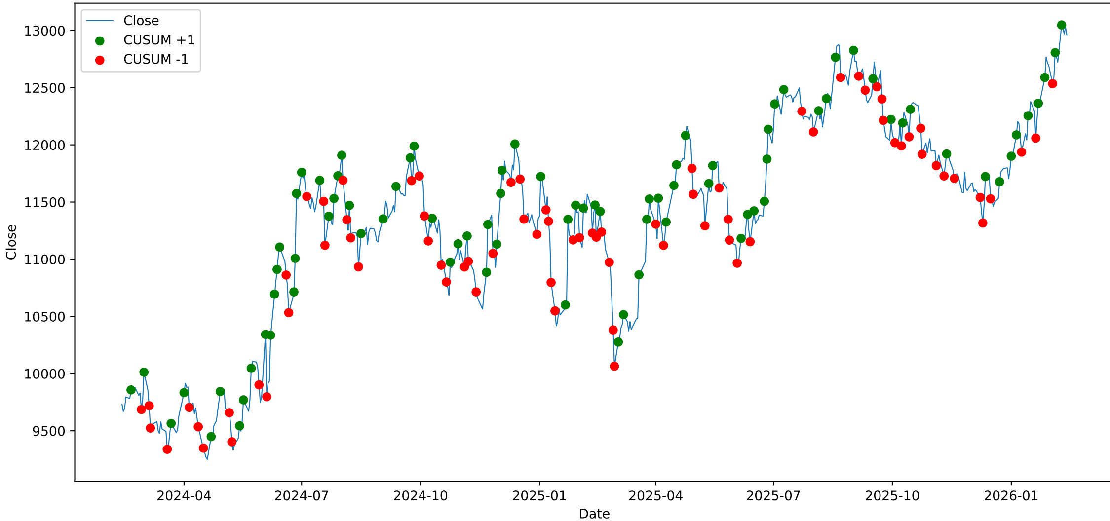
ULTRACEMCO - Close with CUSUM Events
