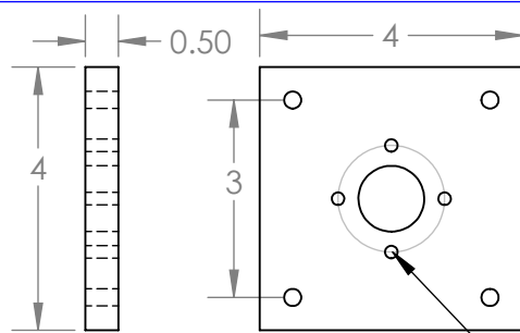
END PLATE
