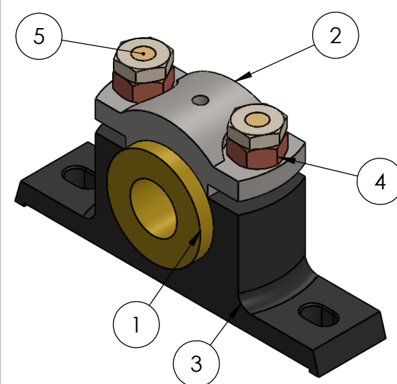
ISOMETRIC VIEW OF PLUMMER BLOCK ASSEMBLY
