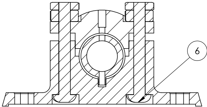
PLUMMER BLOCK ASSEMBLY
