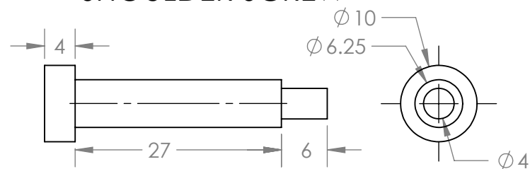
SHOULDER SCREW
