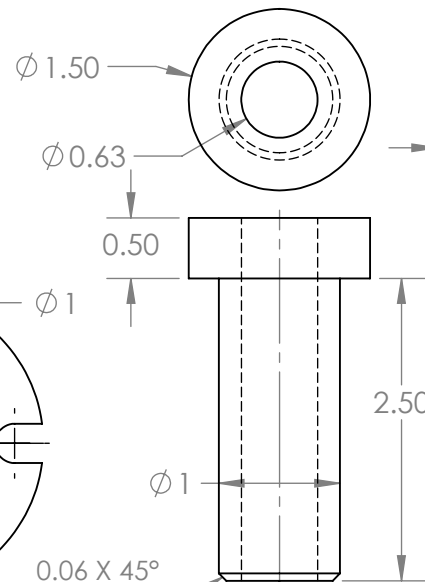
CENTER PIN
