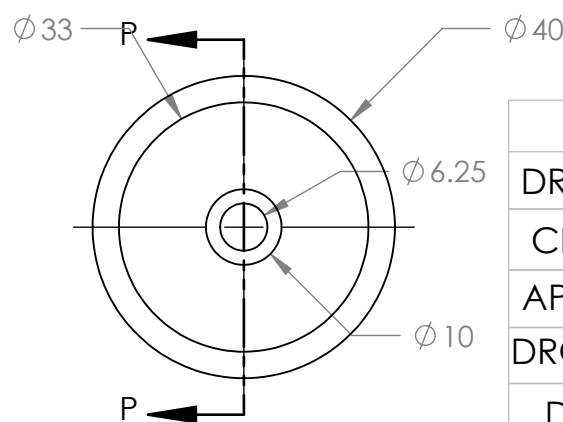
WHEEL
