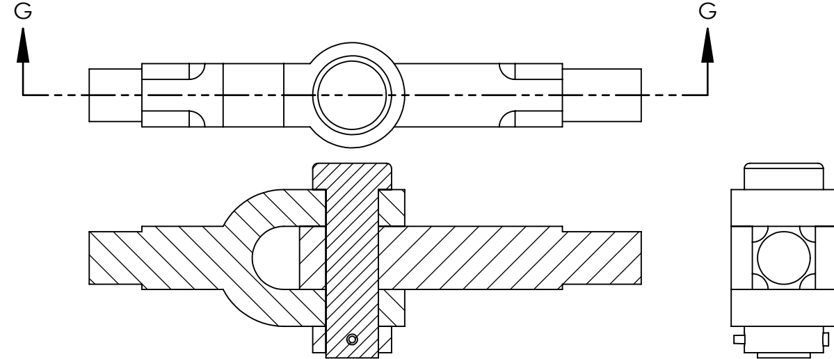
NUCKLE JOINT ASSEMBLY
