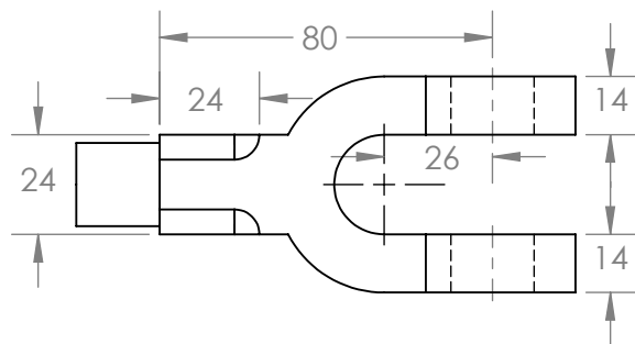
FORK END
