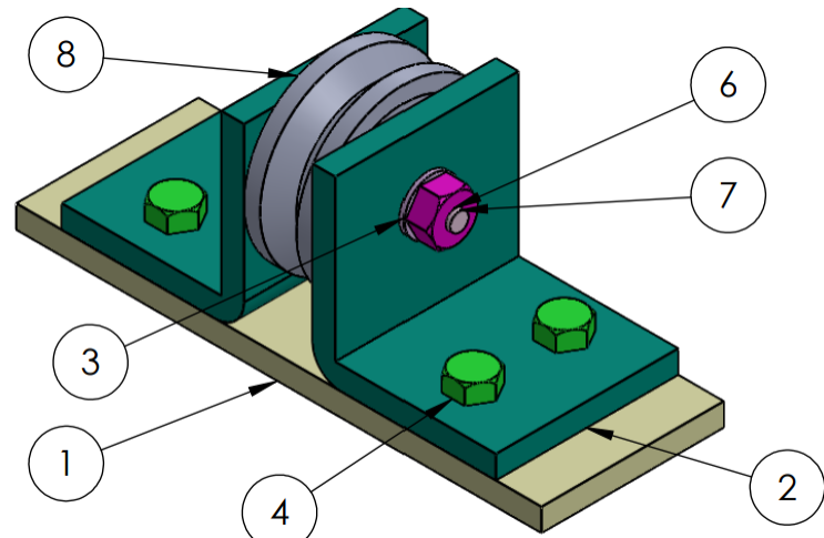
WHEEL SUPPORT ASSEMBLY
