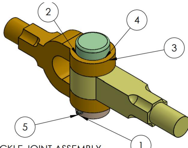
KNUCKLE JOINT ASSEMBLY
