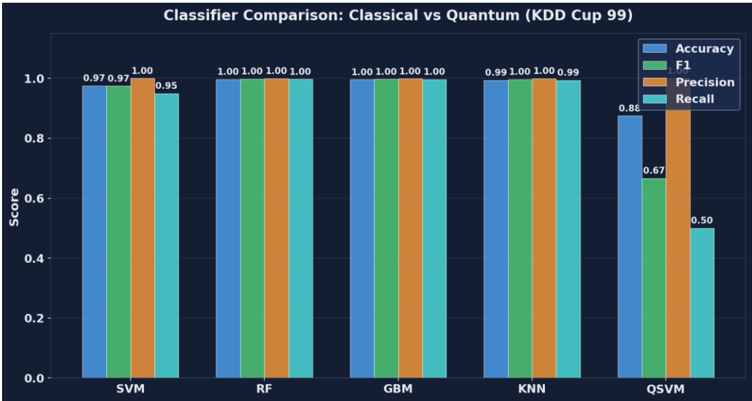
Figure 9.1: Per-method classifier comparison on KDD Cup 99 (30 runs). Random Forest reaches F1 = 0.998 against QSVM at 0.667.
