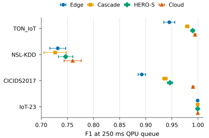
Fig. 3. Closest-baseline comparison at 250 ms QPU queue time. HERO-S improves over edge-only and the uncertainty cascade while remaining below the average latency budget.
