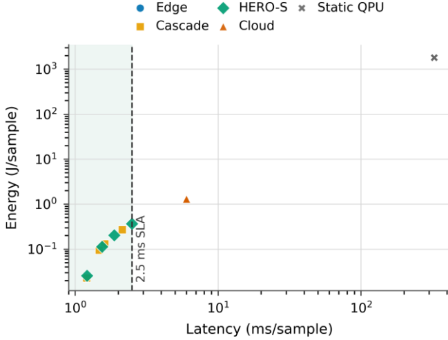
Fig. 6. Energy-latency policy tradeoff. The dashed line marks the 2.5 ms/sample average budget.
