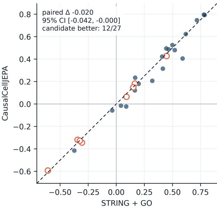
d Systema Pearson · target excluded vs. STRING + GO
