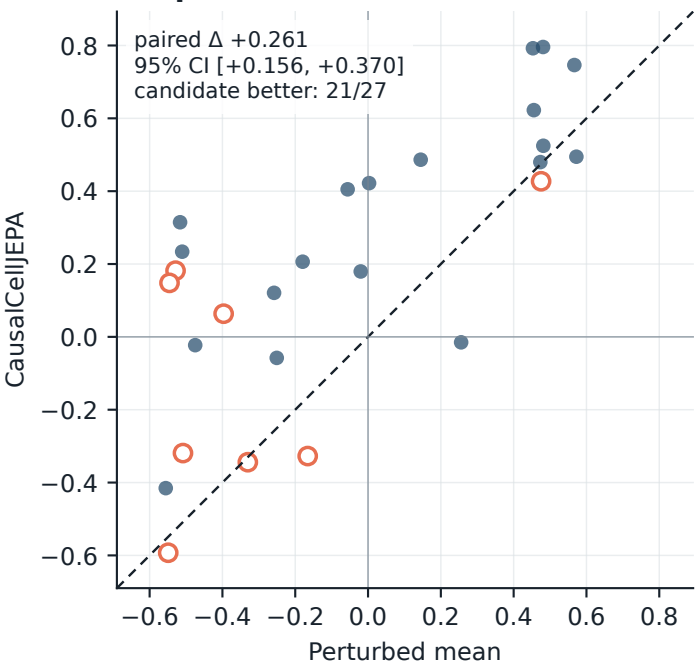
c Systema Pearson · target excluded vs. perturbed mean
