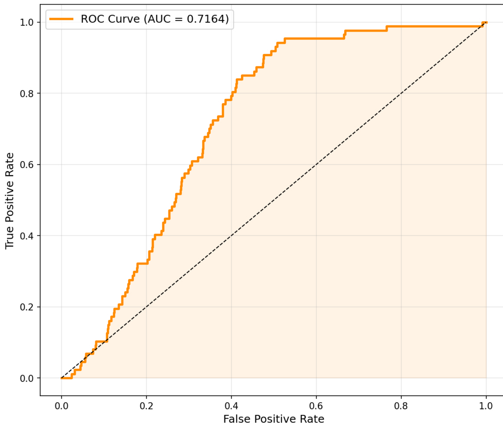
ResNet50 — ROC Curve
