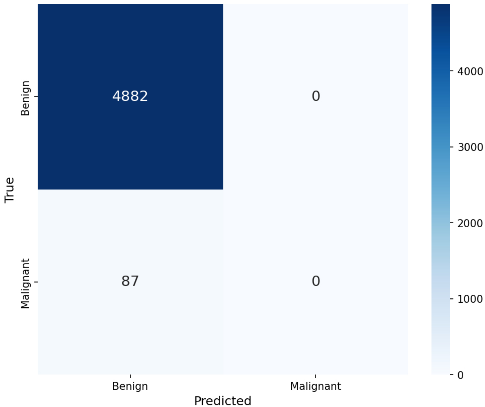
ResNet50 — Confusion Matrix
