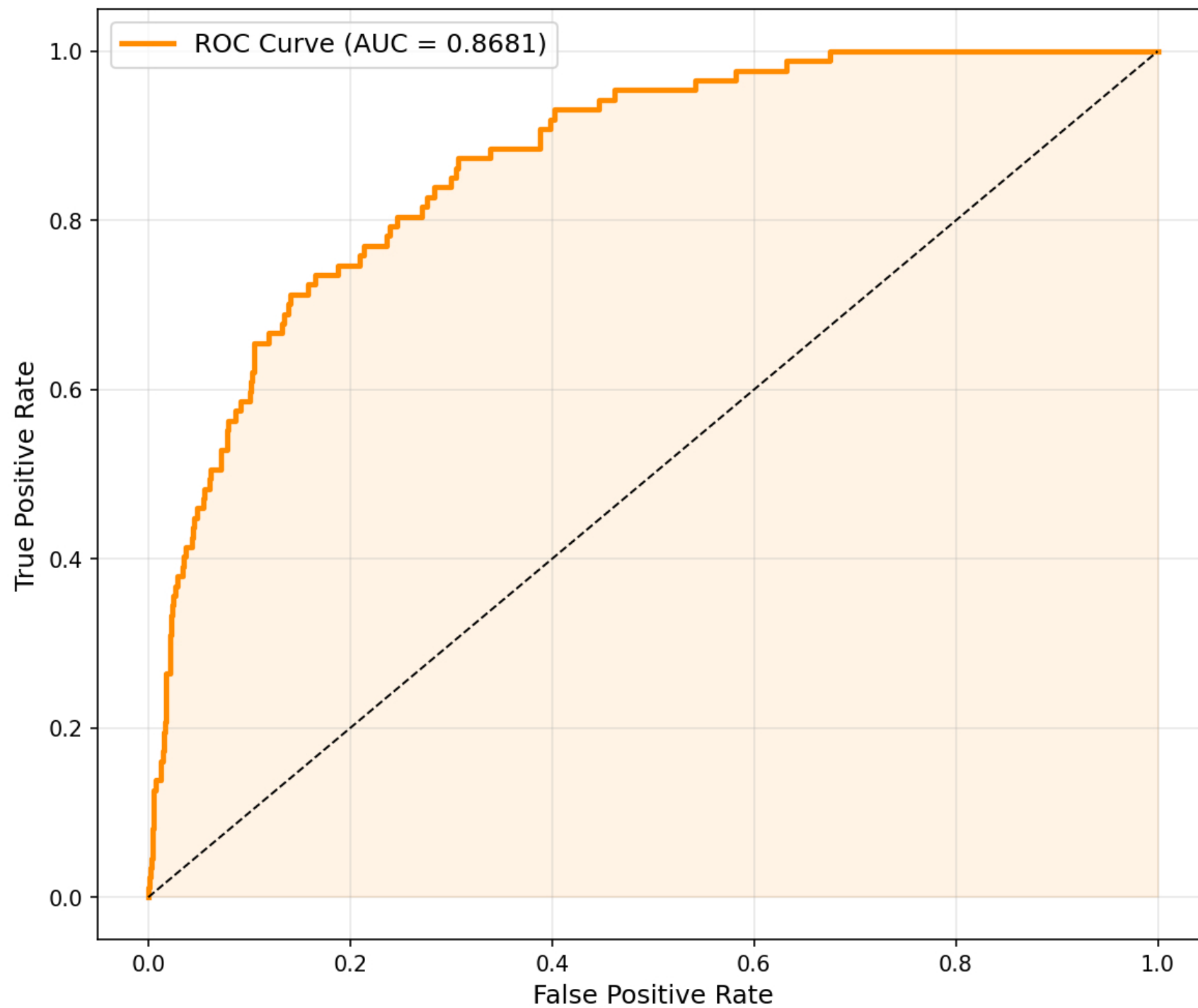
MobileNetV2 — ROC Curve
