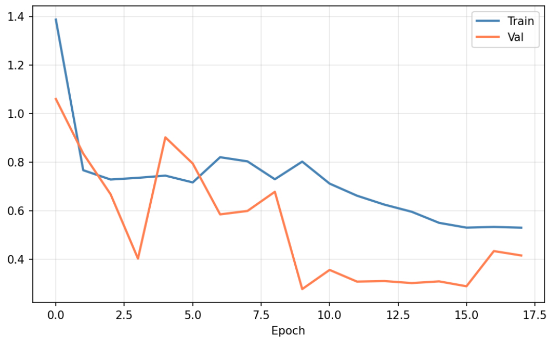
Loss
