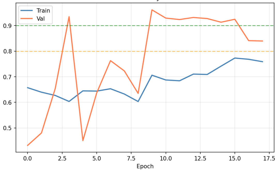
Accuracy
