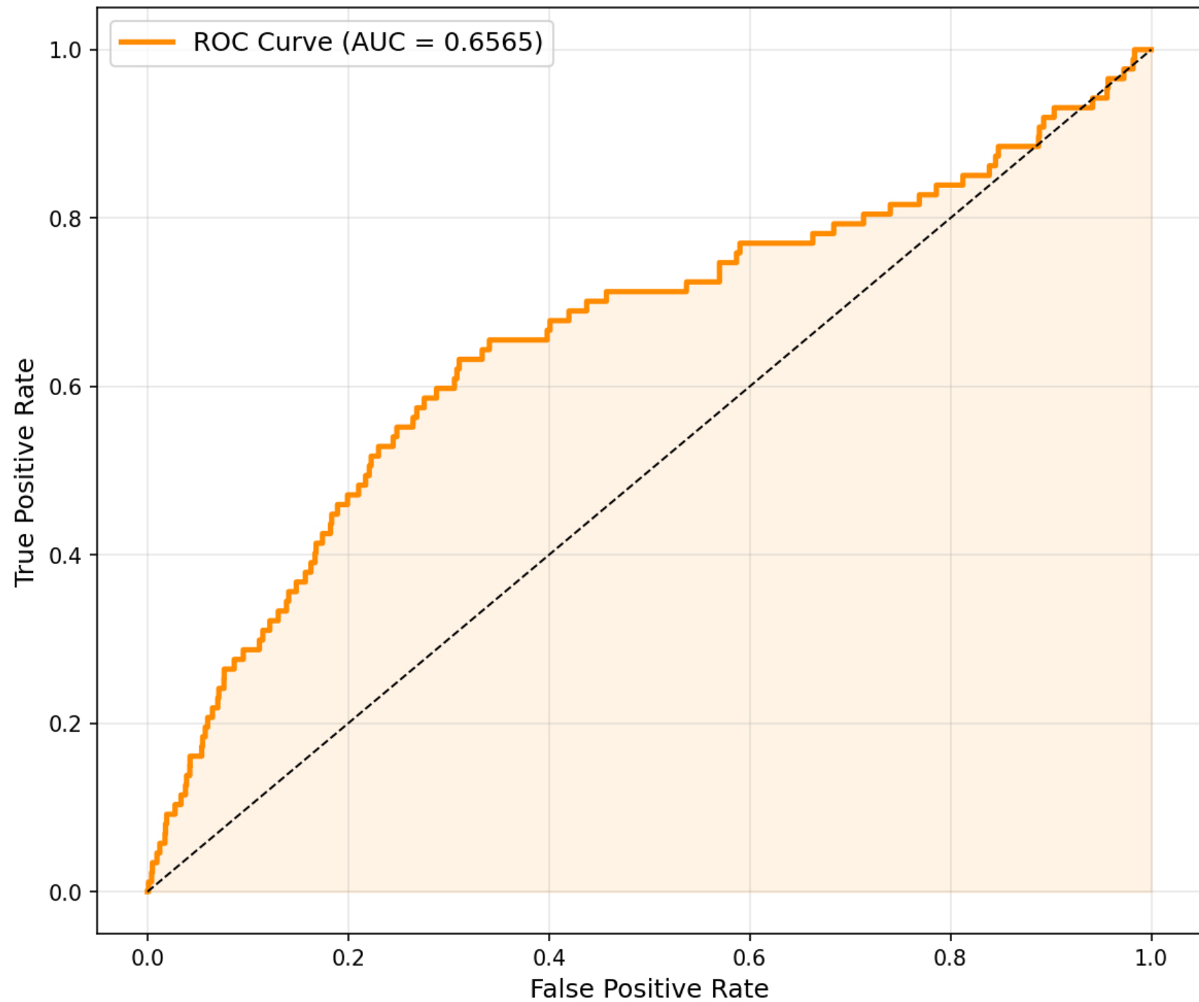
EfficientNetB0 — ROC Curve
