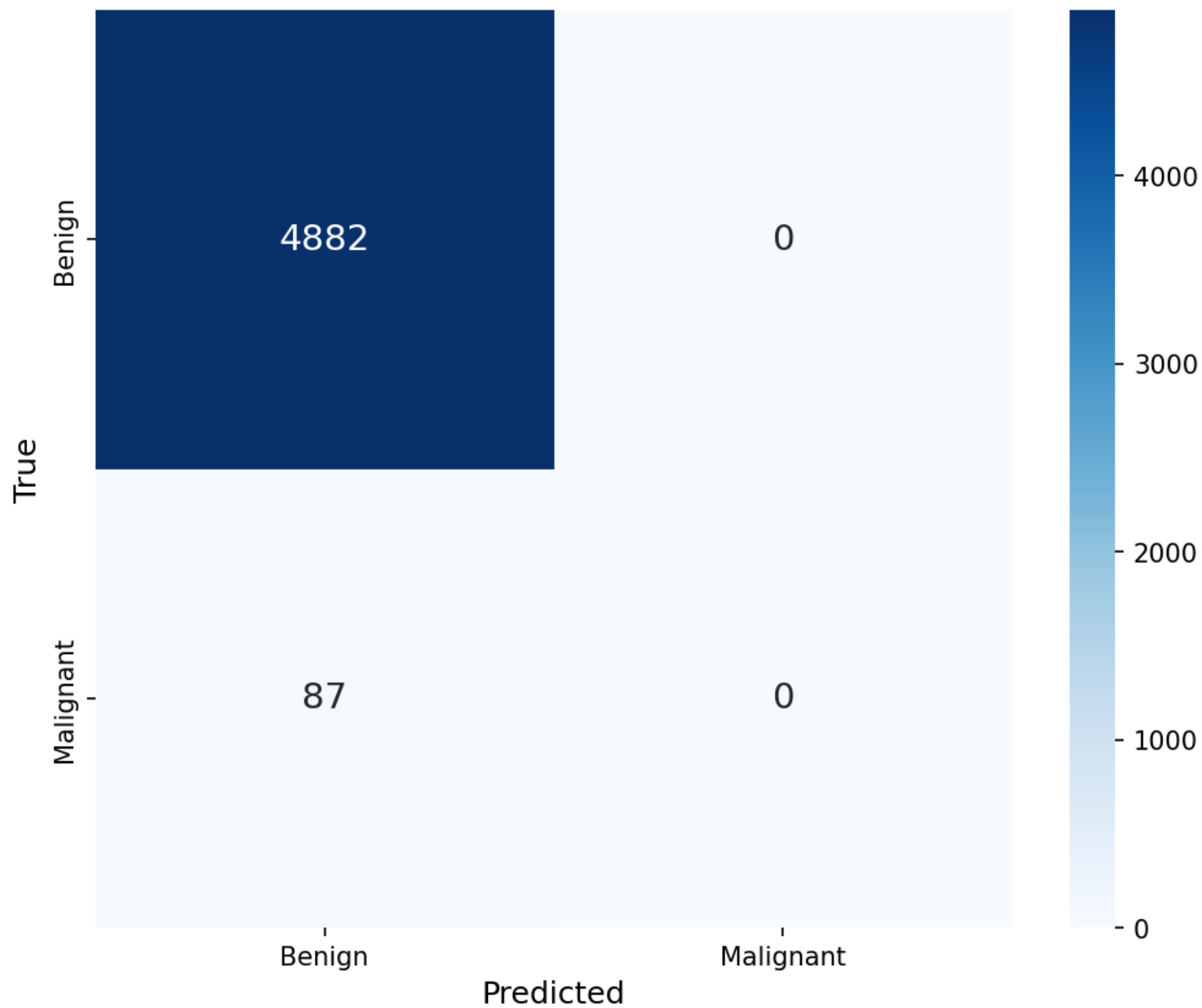
EfficientNetB0 — Confusion Matrix
